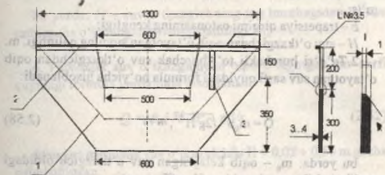
2.33-rasm. Trapetsiya shaklidagi Chippoletti (VCh-50) suv o'lchagichi: (vodoslivi), tubining kengligi 500 mm (50 sm, 1 sm-10 mm)
