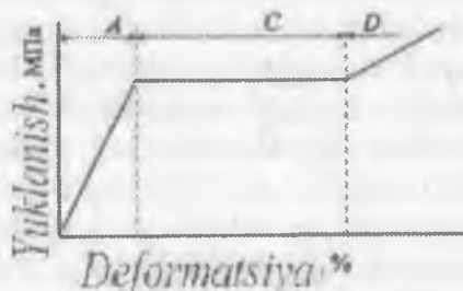
16. 9-rasm. Kristallik polimerni cho'zish diagrammasi.
