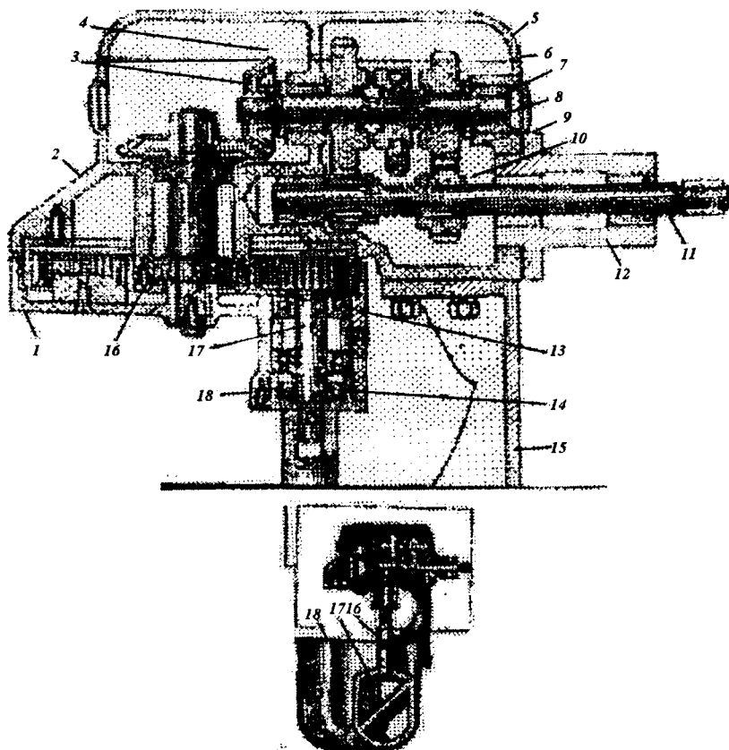
7.8-rasm. MSM-7-8-20 markali ko‘pish bajaradigan mexanizm:
