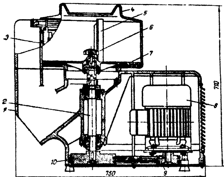
5.13-rasm. SKM-400-1200 markali sabzavot mahsulotlarini kesuvchi jihoz.
