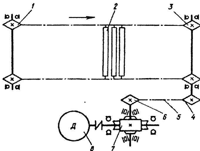
4.3-rasm. MSM jihozning kinematik chizmasi:
