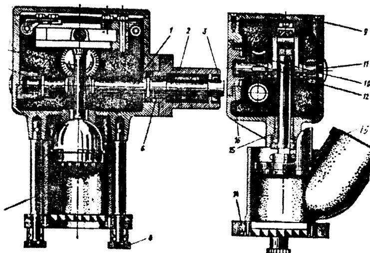
5.15-rasm. MO-28-100 markali kartoshka kesish uchun mo'ljallangan jihoz.
