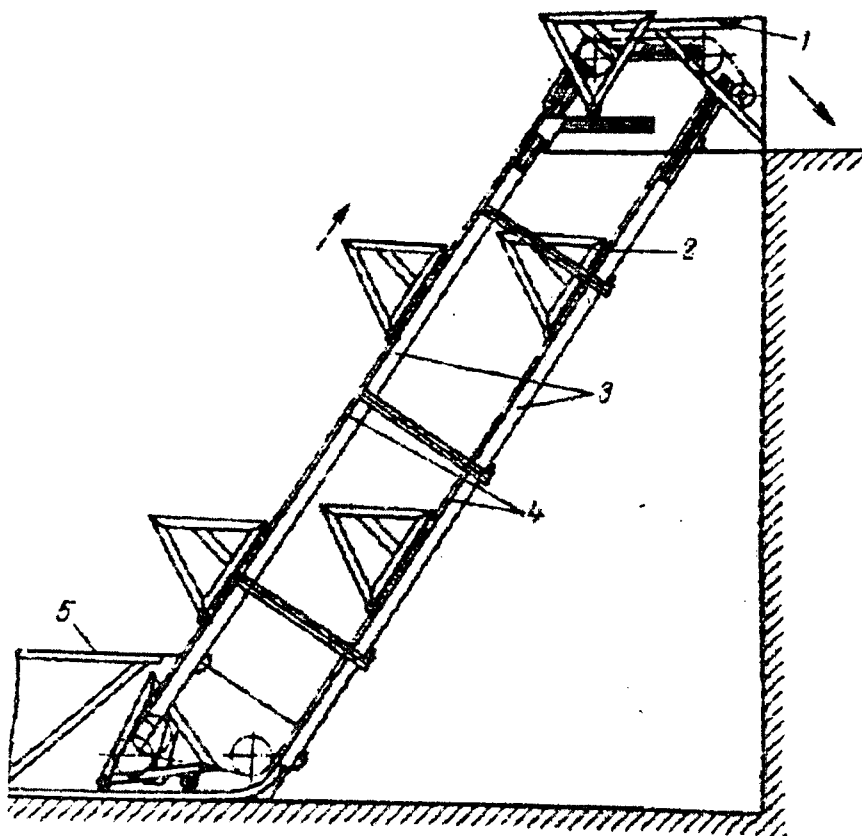
11.23-rasm. Qiya polkali elevator EPN-1.
