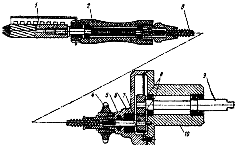
3.9-rasm. BT IMI markali baliqlarni tangachalardan tozalaydigan moslama.
