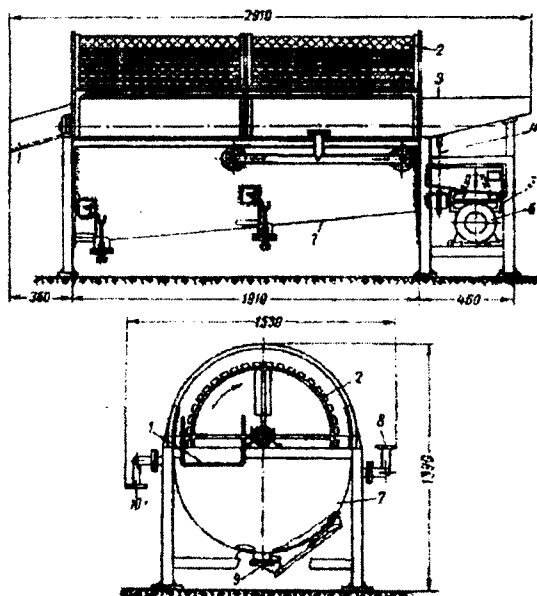
2.2-rasm. Barabanli yuvish jihozlari
