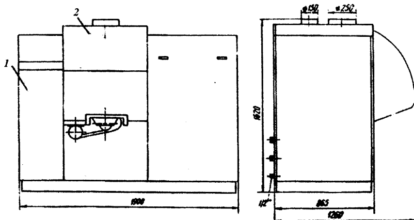
7.12-rasm. Bug' bilan isitiladigan aralashtirgich.
