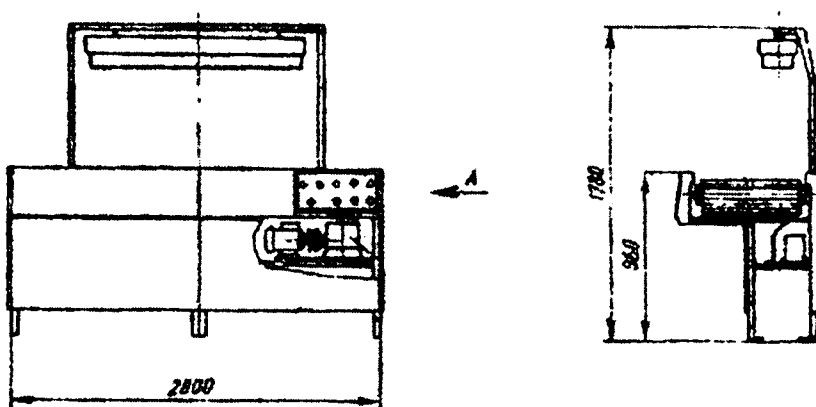
4.7-rasm. MPO-2 markali ajratuvchi mashina.
