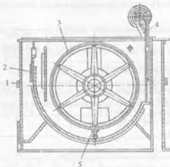
5.6-rasm. ЦҚБ-04 rusumli shabersiz quyultirgich
