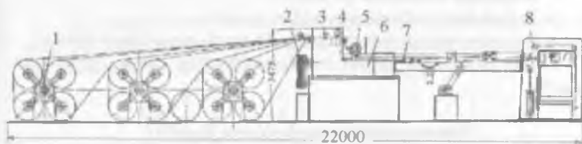
10.15-rasm. C1-13 rusumli polotnoni ko'ndalangiga qirqish dastgohi:
