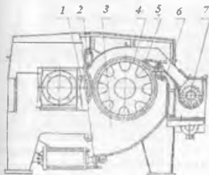
5.3-rasm. C2Б-07-35 rusumli ikki barabanli quyultirgich:
