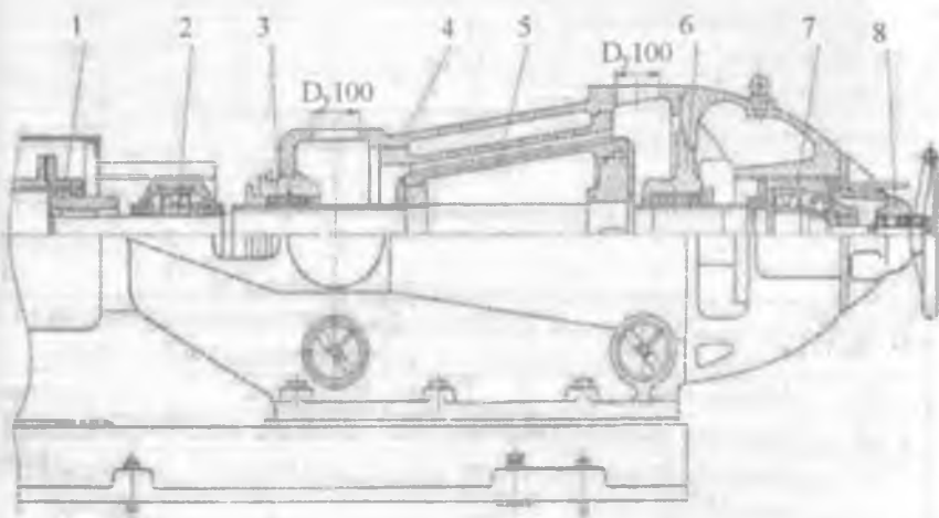
2.15-rasm. MKЛ-01M rusumli konusli tegirmon:
