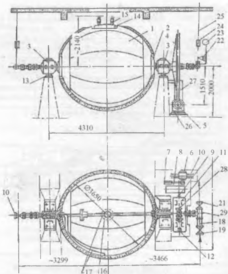
1.10-rasm. Shar shaklidagi QJ25 rusumli pishirish qozoni:
