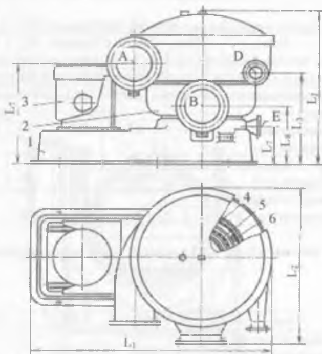
6.1-rasm. Y3-09-01, Y3-12, Y3-13 rusumli yopiq tugun tutgichlar: 1 – plita; 2 – korpus; 3 – dvigateli; 4 – tashqi to'rt; 5 – ichki to'rt; 6 – parrak.
