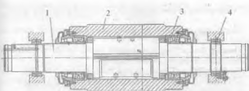
8.5-rasm. Erkin harakatlanadigan val:
