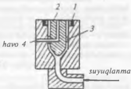
7-rasm. Burchakli halqasimon kallak sxemasi:
