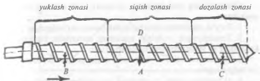
4-rasm. Chervyakning zonalarga bo'linishi.
