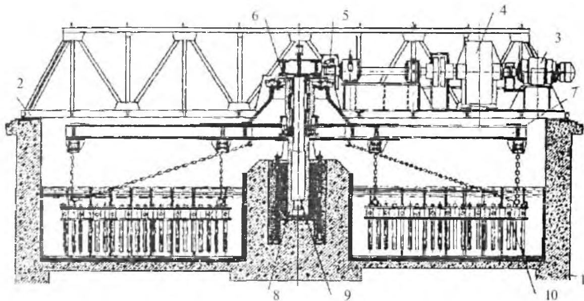
4-rasm. Aralashtirgich:
