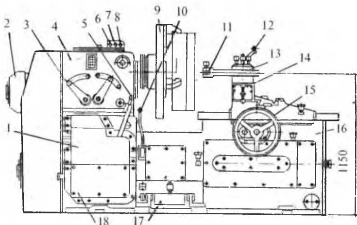
6-rasm. 1S51N mufta charxlash stanogi:
