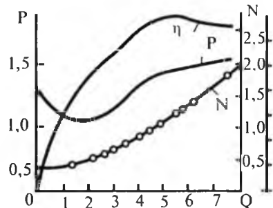
15-rasm. Ventilatorning o'ziga xos ( individual) tavsifi.
