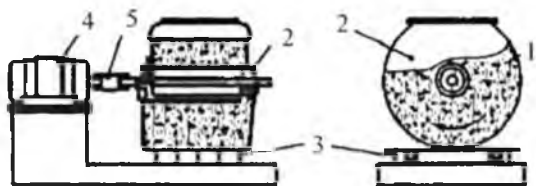
22-rasm. Tebranma tegirmonning gratsion turi:
