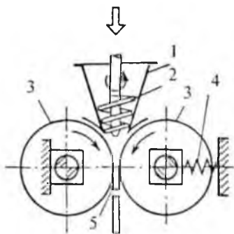
40-rasm. Jo'vali donalagich sxemasi:
