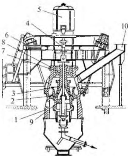
3-rasm. Ekssentrik konusli (yoki inersion) maydalagich:
