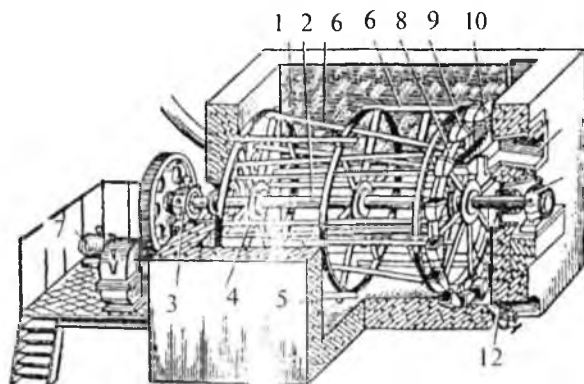
6-rasm. Kovshli aralashtirgich:
