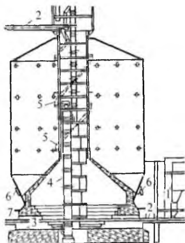
5-rasm. Silosli ombor:
