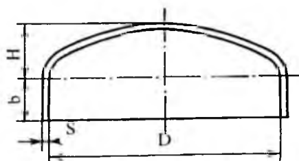
3-rasm. Ellipssimon tub.
