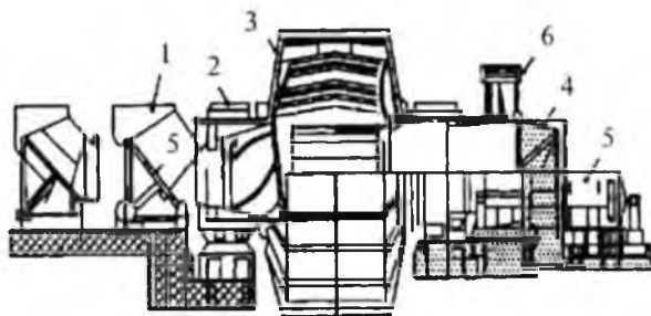
20-rasm. «Aerofol» barabanli tegirmon: 1 – ta'minlovchi moslama; 2 – tebranuvchi moslama; 3 – baraban; 4 – elak; 5 – elektryuritgich; 6 – gardishli shesterna.
