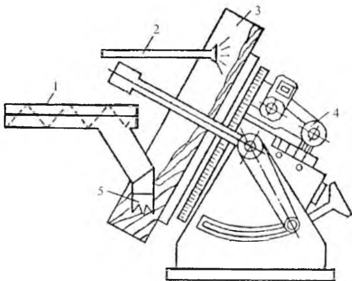
7-rasm. Tarekasimon donalagichning tuzilishi.
