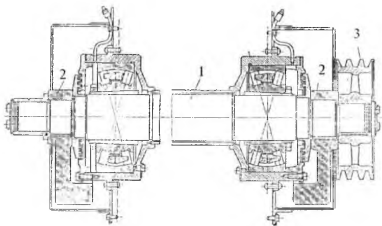
5-rasm. Vibroval.
