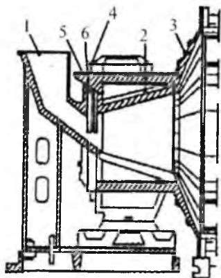
6-rasm. Sapfa bo'shlig'ida voronka bor tegirmonning material solish qismi:
