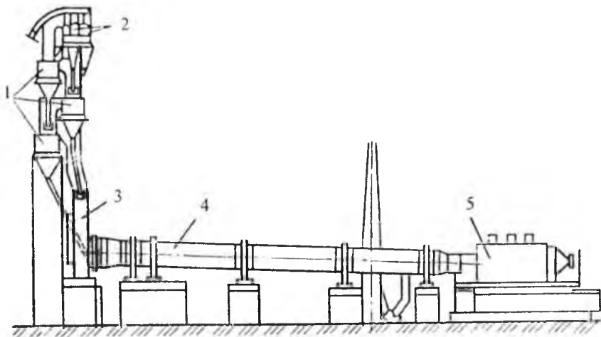
4-rasm. Siklonli issiklik almashtirgichli aylanma pech:
