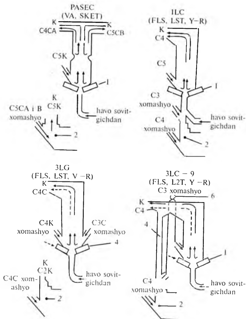
IV guruh: 1 – asosiy gorelkalar; 2 – aylanma pech; 3 – qo'shimcha gorelkalar; 4 – dempferlovchi qopqoq; 5 – tiklovchi zona; 6 – bo'lgich.
