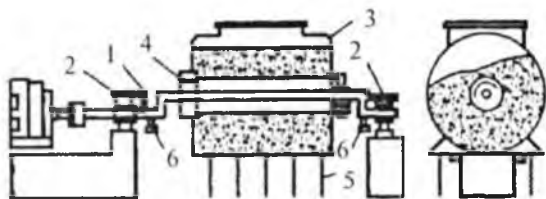
22-rasm. Tebranma tegirmonning gratsion turi:
