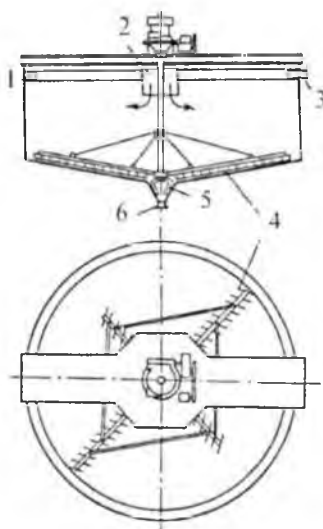
1-rasm. Suspenziyani markazdan uzatadigan tipa-voy tindirgich:
