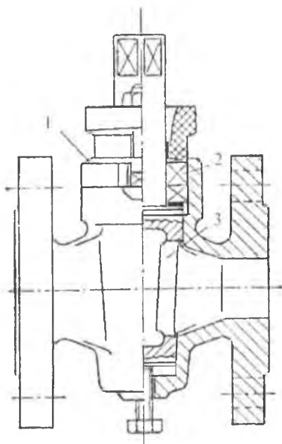
23-rasm. Cho'yandan yasalgan flantsi bor salnikli o'tish jo'mragi: 1 — korpus; 2 — salnik; 3 — tiqin.
