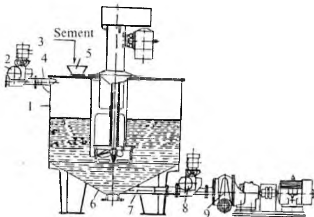
9-rasm. Asbestsment massasi tayyorlovchi turboaralashtirgich sxemasi: 1 – korpus; 2 – klapan; 3 – elektr yuritgich; 4 – truba; 5 – voronka; 6 – tag qism; 7 – patrubok; 8 – klapan; 9 – nasos.
