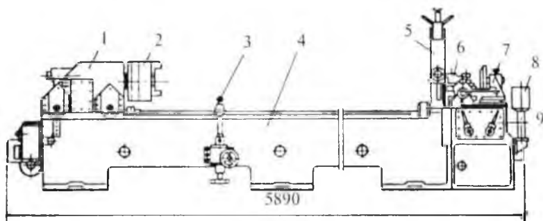
5-rasm. Mufta qirquvchi IS49N:
