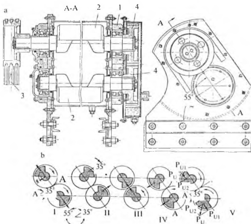
14-rasm. Vibrator:
