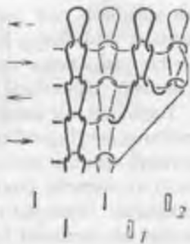
4.15-rasm. Ribana 1+1 asosida (uchinchi variant) ikkala ignadondan bittadan igna qo'shib hosil etilgan gardish tuzilishi.
