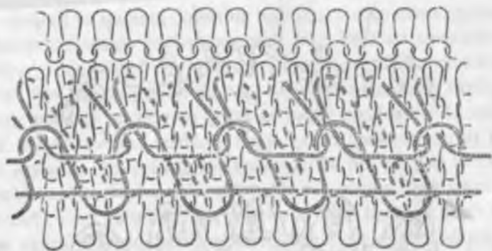
2.6-rasm. Ripshaybasiz paypoq to'quv avtomatida to'qilgan paypoqning bortini birlashtiruvchi chok tuzilishi (overlog mashinasida choklangan).
