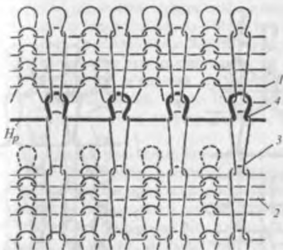
3.2-rasm. Ajratish qismidagi maxsus ajratish ipining to'qimadagi tuzilishi.
