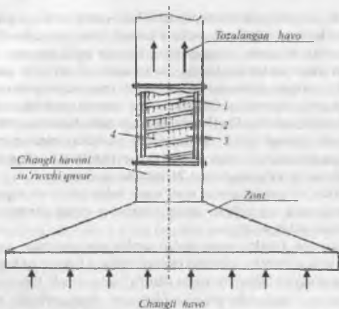
4.25-rasm. Filtrlovchi vositani o'rnatish sxemasi:
