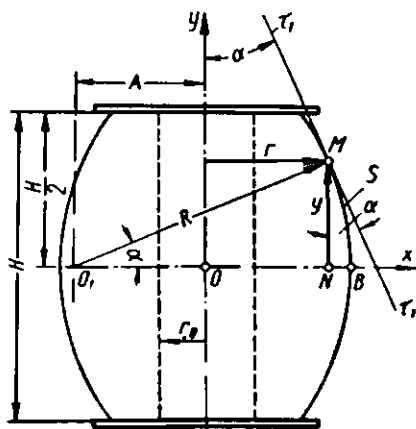
3.5- rasm. Sferoid o'ralish.
