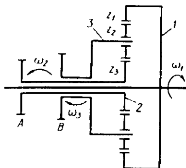
17.2-rasm. Pilik mashina differensial sxemasi.
