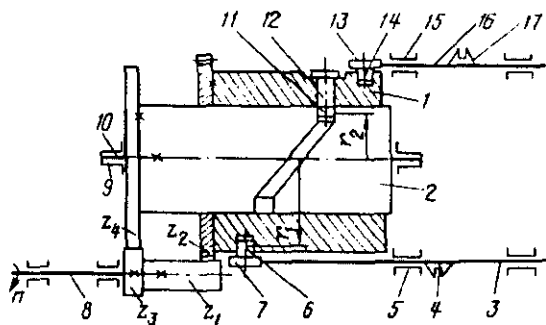
2.9- rasm. Qavatli eshuv mashinasi:
