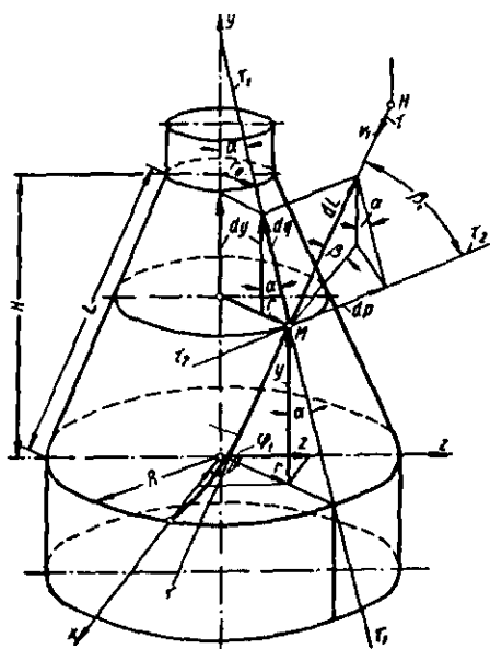
3.4- rasm. Konussimon o'ralish.
