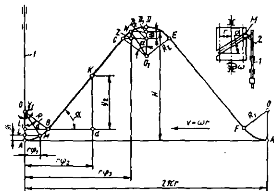
14.5- rasm. Ariqchali silindrik mushtcha nazariy shaklchizig'ining yoyilmasi.
