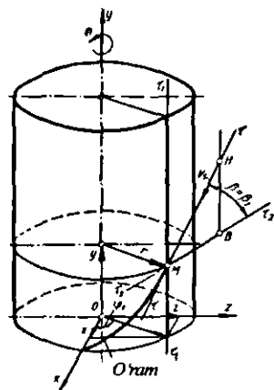
3.2- rasm. Silindrik o'ralish.
