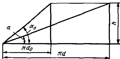
10.6-rasm. Ip o'ramining yoyilmasi:
