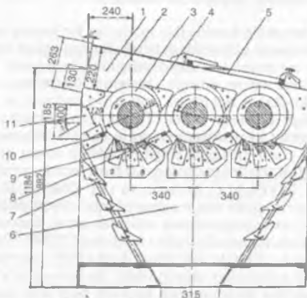
1.17-rasm. 1VP rusumli tola tozalagich:
