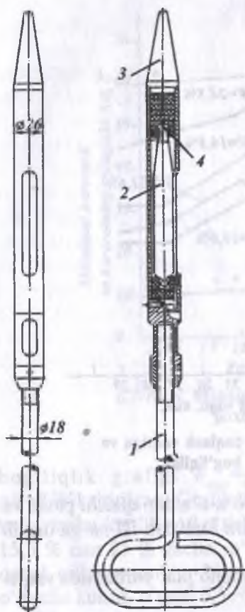
38-rasm. Termochop.
