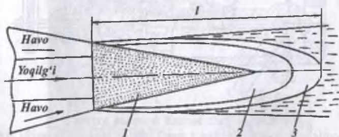
8.5-rasm. Suyuq yoqilg'ining alanga olishi:
