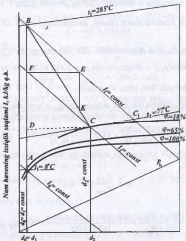
5.6-rasm. I - d diagrammada qurish jarayoni.
