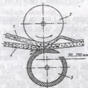
31-rasm. Odatdagi ikki valli pressdagi vallarning joylanishi:
