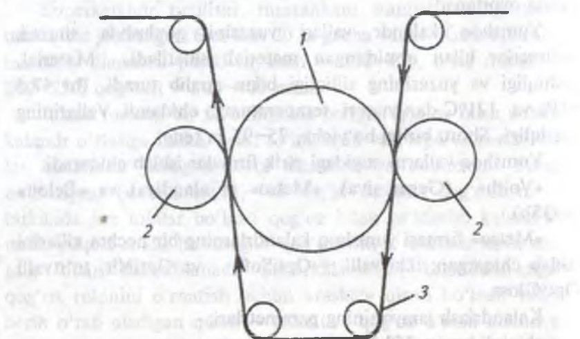
53-rasm. Loshlovchi kalandr sxemasi:
