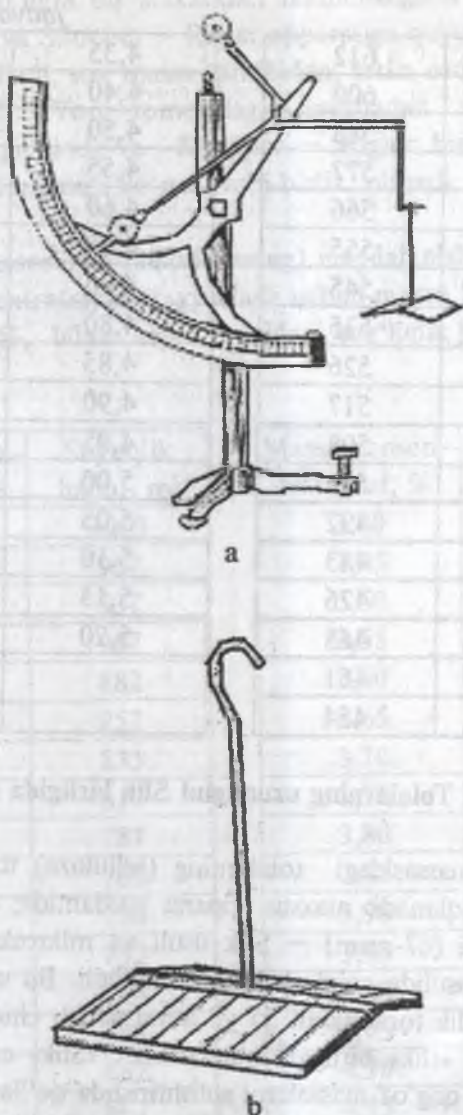
67-rasm. Massadagi tolalarning o'rtacha uzunligini aniqlovchi pribor:
