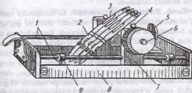
69-rasm. Qog'ozning yelimlanish darajasini aniqlovchi
