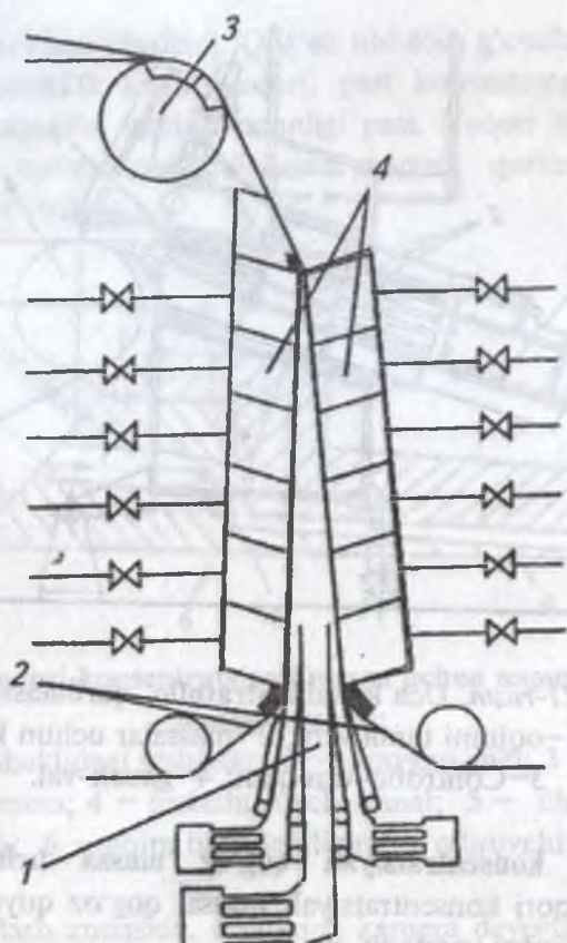
20-rasm. Controflo-Foemier shakllantiruvchi qurilmasining sxemasi:
