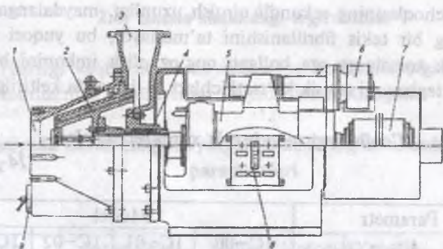
5-rasm. Konus shaklidagi 1C-01 modelli Conflo tegirmoni:
