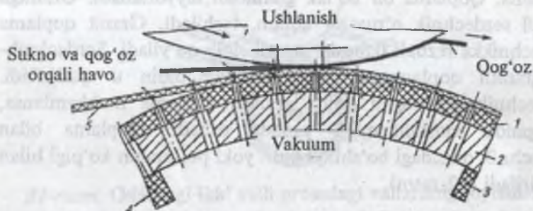
33-rasm. So'ruvchi pressda qog'oz polotnmoni presslash:
