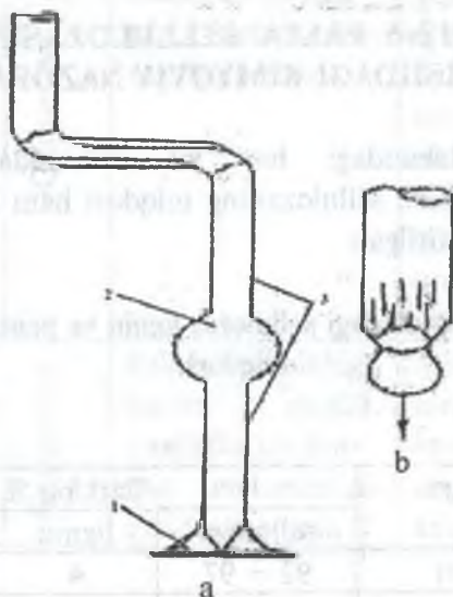
63-rasm. Sirt tortish kuchini aniqlashda qo'llaniladigan stalagmometr:
