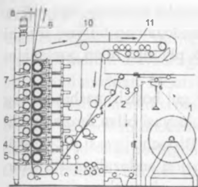
208-rasm. Gul bosish agregatining texnologik sxemasi:
