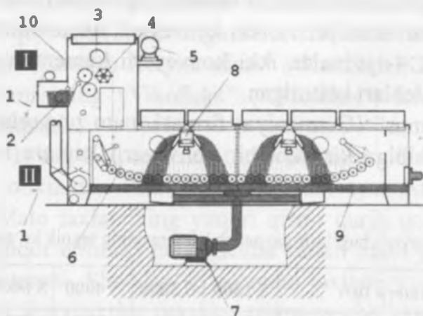
46- rasm. "Moenus" firmasining bug'lash-qaynatish kamerasi:
