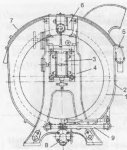
139- rasm. KB – 50 – 1 bo'yash barabanining sxemasi:
