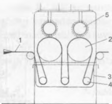
75- rasm. “Menzel” firmasining yuvish-tozalash mashinasidan mato oʻtish sxemasi:
