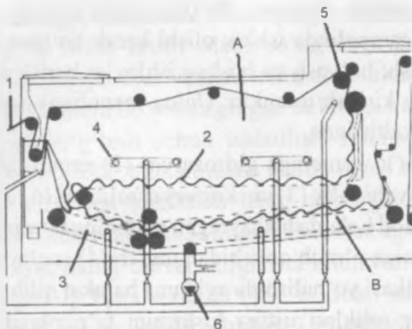
45- rasm. "Ramish Kleynefers" firmasining bug'lash-qaynatish kamerasi.
