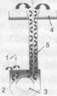
67- rasm. Matoni tor tirqishdan o'tishda yuvish sxemasi:
