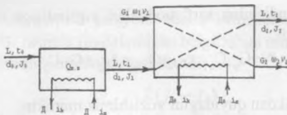
193- rasm. Quritish uskunasiining prinsipial sxemasi: 1 – isitgich; 2 – quritish kamerasi; 3 – qo'shimcha isitgich.
