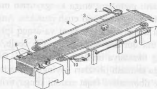
112- rasm. Zanjirli mato kengaytirish mashinasining sxemasi:
