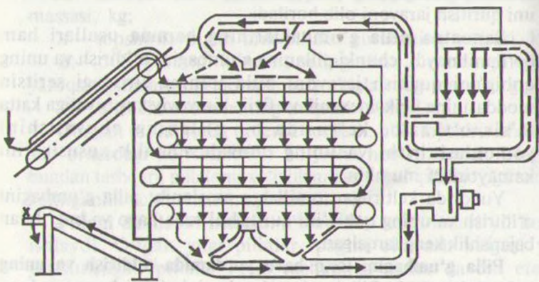
4.4-rasm. KSK-4,5 rusumdagi pilla quritish mashinasi.
