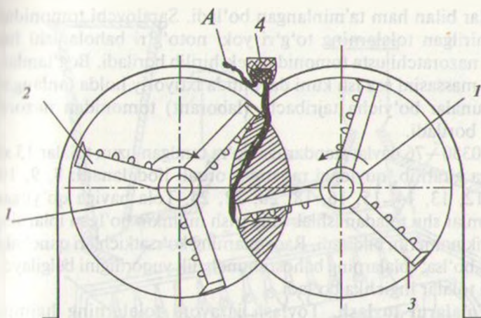
3. 10-rasm. MT-100L titish mashinasining sxemasi:
