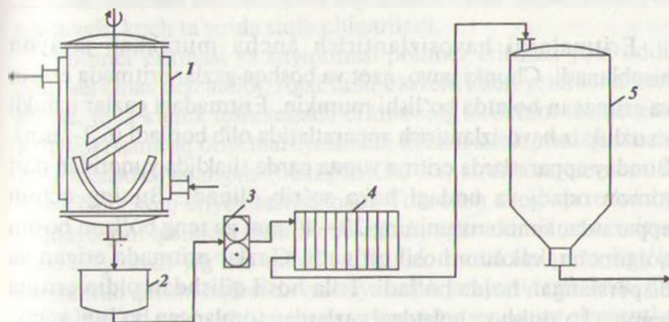
6.1-rasm. Polimerni eritish va uni filtrlab tozalash sxemasi: 1—eritish baki; 2—filtr-ushtagich; 3—nasos; 4—filtr; 5—oralik bak.
