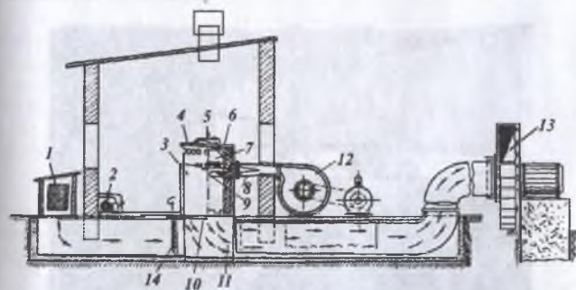
8.2-rasm. TJK-1,5 rusumli issiqlik generatorining sxemasi: 1-filtr; 2-nasos; 3-qobiq; 4-eshikcha; 5-qopqoq; 6-o'tga chidamli maxsus g'isht; 7-yanish kamerasi; 8-quvur; 9-kuzatish oynasi; 10-yanish jarayonini tugallash vositasi; 11-aralashtirish kamerasi; 12-ventilator; 13-tutun so'rg'ich; 14-panjarali qopqoq.
