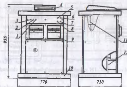
9.3-rasm. YCX-1 rusumli termonamo'lgach:
