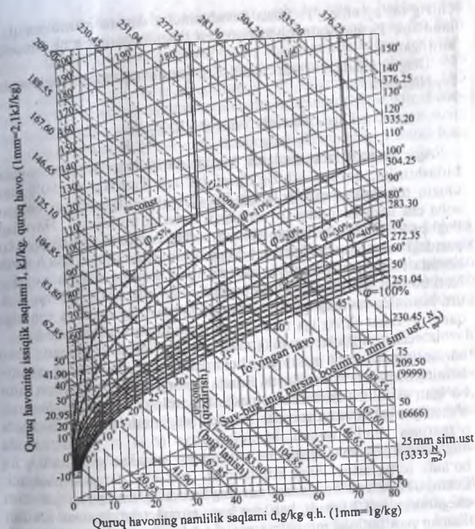
2.1- rasm. Nam havoning I-d diagrammasi.
