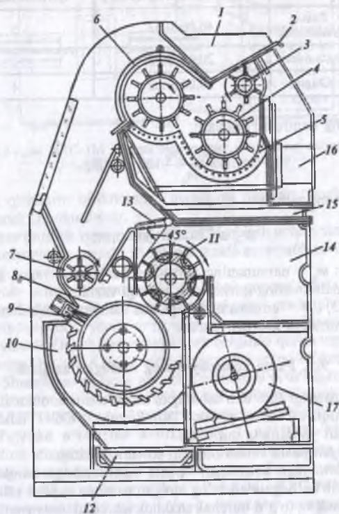
9.5-rasm. JKM rusumli asbob chizmasi:
