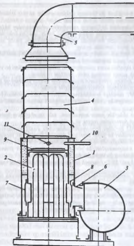
9.7-rasm. CXJI-3 rusumli laboratoriya quritkichi: 1-quritkichning asosi; 2-quvvatli energoisitgich elementlari HB-6-1,2/1,0; 3-ventilator - 2BP -2; 4-paxta xomashyosi namunalarini joylashtirish kassetasi; 5-so'rish moslamalari; 6-ventilatorli diffuzor; 7-ichki silindr; 8-gorizontaal tirqishlar; 9-ikki tomonlama ekranli to'r (peshirka); 10-simobli termometr; 11-ikki metalli issiqlik relesi.
