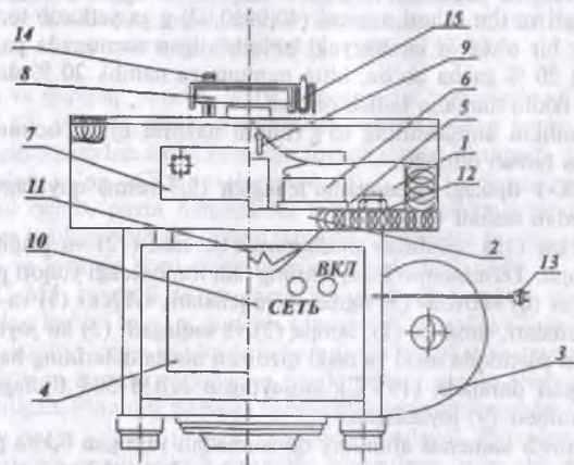
9.2-rasm. IIICX-1 rusumli quritish javoni sxemasi:
