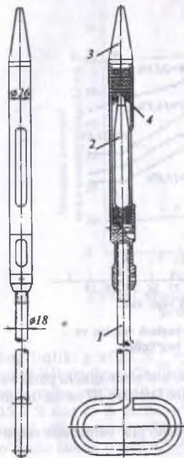
38-rasm. Termochop.
