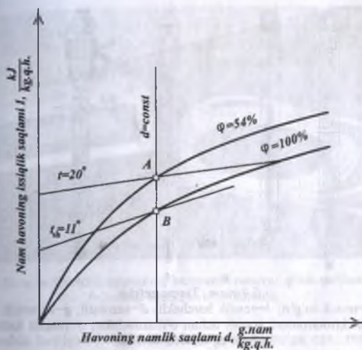
2.7-rasm. Shabnam nuqtasini I - d diagrammasida aniqlash.
