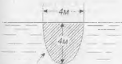
Parabola 9.30- rasm
