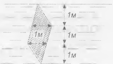
Parallelogram
