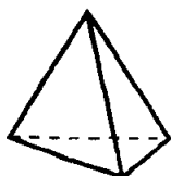
Tetraedr
