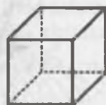
kub
