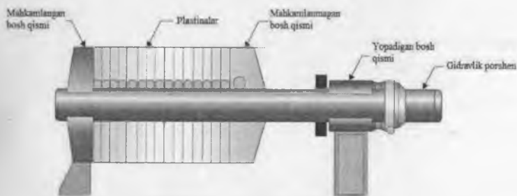
90-rasm. Plastinali filtr press sxemasi (U.S. EPA (1979) pg. 9–53.
