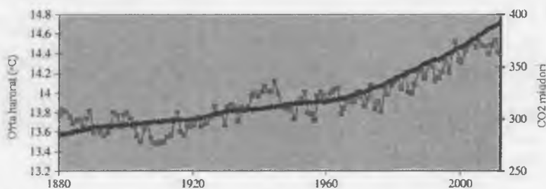
21-rasm. \text{CO}_2 miqdoriga nisbatan global harorat.
