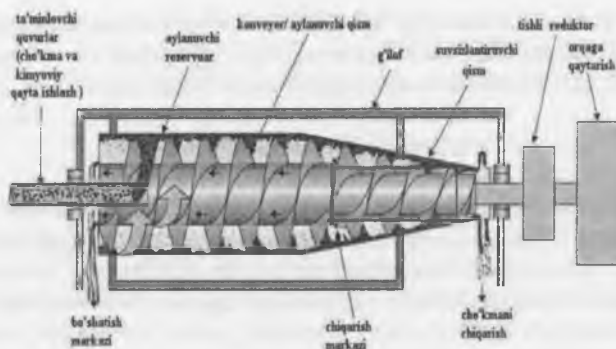
58-rasm. Mustahkam sig'imli uzluksiz parallel sentrifugal.
