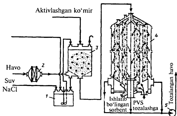
15.1-rasm. Ventilatsion tashlamalarni demerkurizatsiyalash absorbsion qurilmasining sxemasi:
