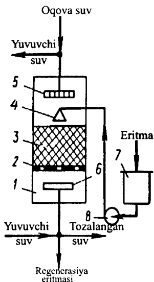
18.16-rasm. Davriy ishlovchi ionalmashish qurilmasining sxemasi:
