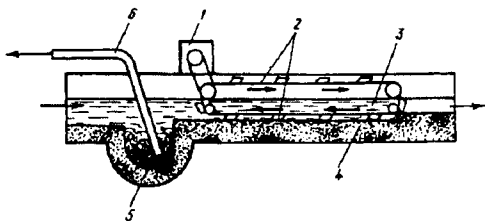
17.2-rasm. Gorizontal qumushlagichning prinsipial sxemasi:
