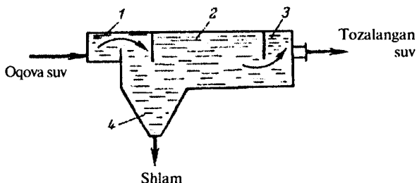
17.3-rasm. Gorizontaal tindirgich:
