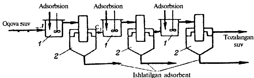
18.10-rasm 1. Adsorbsion qurilmaning sxemasi:
