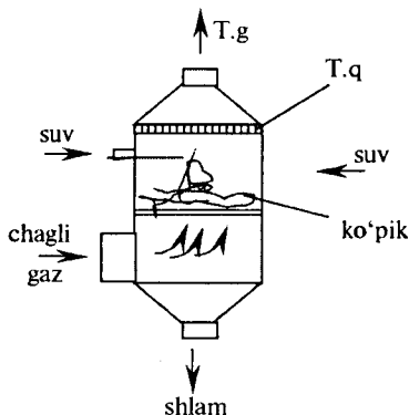
5.10-rasm. Ko‘pikli gazyuvgich:
