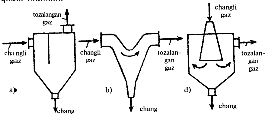
5.2-rasm. Inersion chang ushlagichlar:
