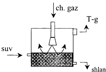
5.11-rasm. Inersion uriluvchi changyutgich.
