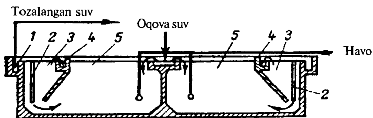
20.3-rasm. Aerotenk:
