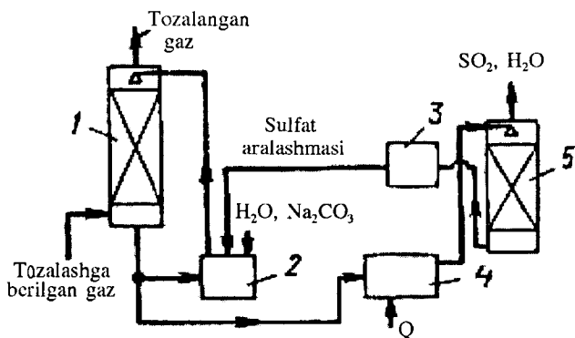
9.7- rasm. Sulfit-bisulfit usulida \text{SO}_2 gazini absorbsion tozalash:
