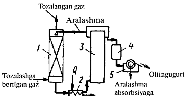
11.2-rasm. Tiloks jarayoni:
