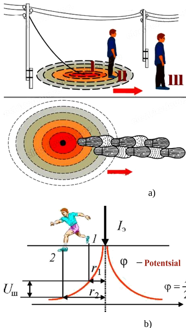
9.3-rasm. Qadamiy kuchlanishning hosil bo'lish sxemasi (a) va potentsiallar farqi hisobi(b) I – kontakt hudud; II- o'ta xavfli hudud; III – xavfsiz hudud;
