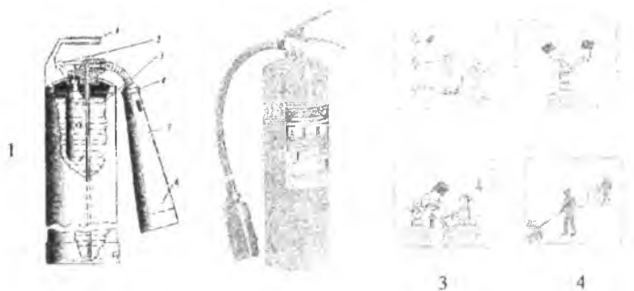
10.8-rasm. OVP-10 markali o't o'chirgichlar va ulardan foydalanish tartibi:
