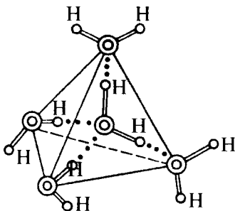
3-rasm. Suvning kristallga o'xshash tuzilishining hosil bo'lishi.
