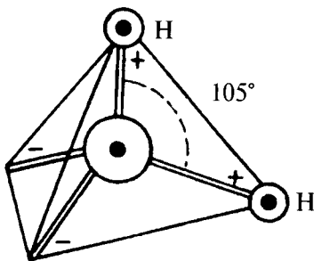
2-rasm. Suv molekulasining tetraedr modeli.
