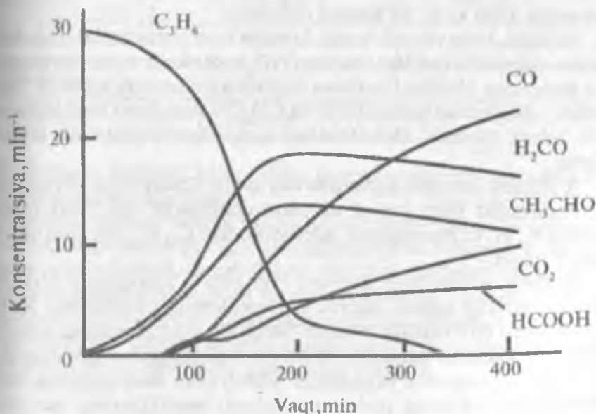
15-rasm. Propilenni nurlantirish ta'sirida o'zgarishi.
