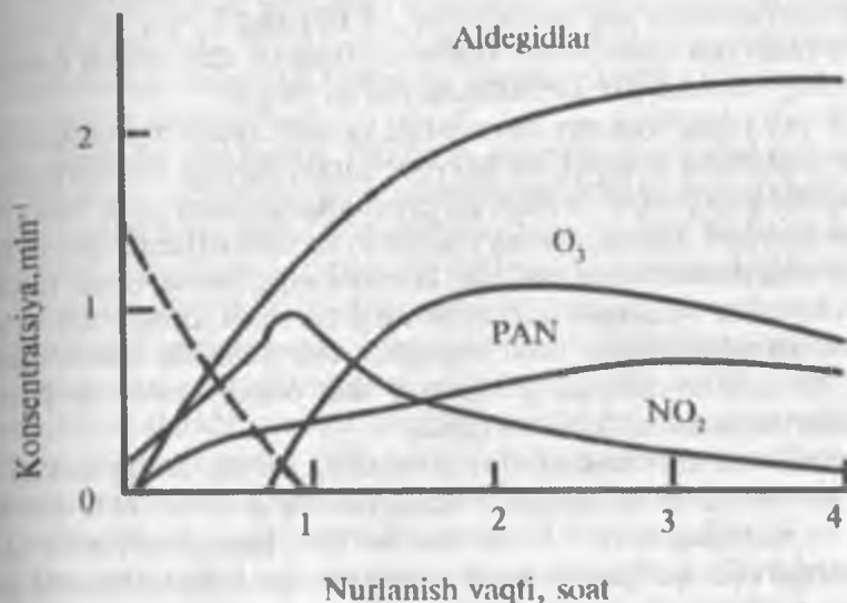
19-rasm. Ifloslantiruvchilarning nurlantirish ta'sirida miqdorining o'zgarishi.
