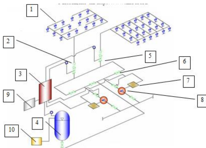
10.6-rasm. Sprinkler qurilmasining ishlash printsiipi
