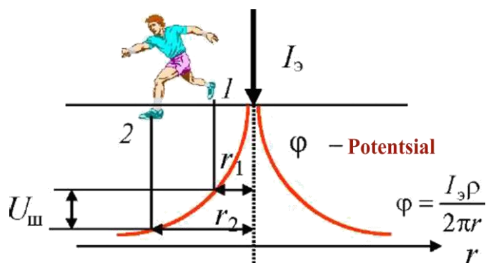
9.3-rasm. Qadamiy kuchlanishning hosil bo'lish sxemasi (a) va potentsiallar farqi hisobi(b) I – kontakt hudud; II- o'ta xavfli hudud; III – xavfsiz hudud;
