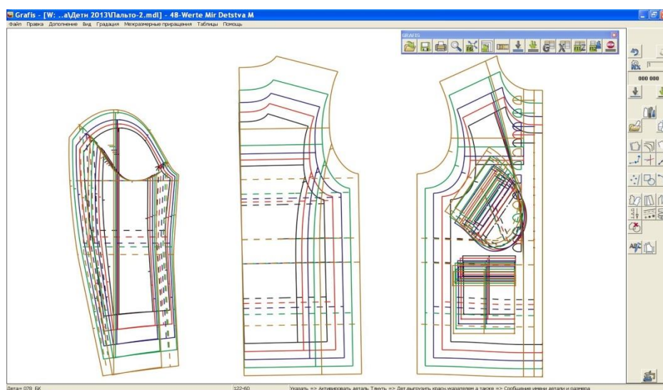
123-rasm. ALTda kiyimi detallarida guruhlash
