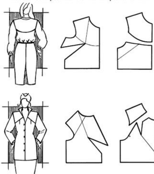
19-rasm. Yelkaga oid va belga oid ayollar kiyimida gorizontaal bo'laklash usulini qo'llab koketkalar modellashtirish
