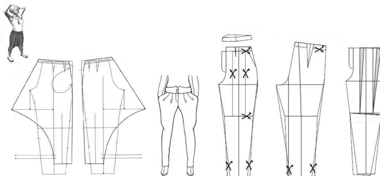
103-rasm. Ayollarning “Golife” bichimdagi modellashtirilgan shimlari
