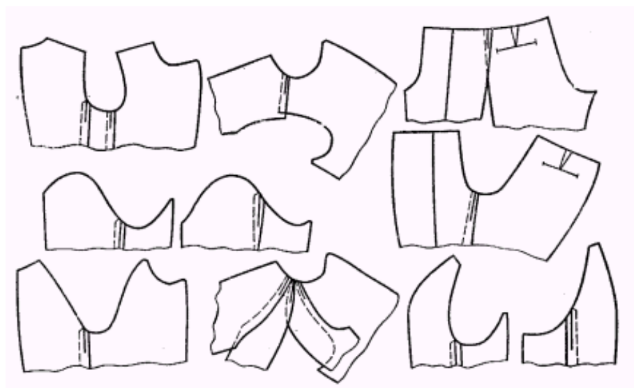
114-rasm. Pdjak (a) va shim (b) detallarning hosila andazalarini tayyorlash
