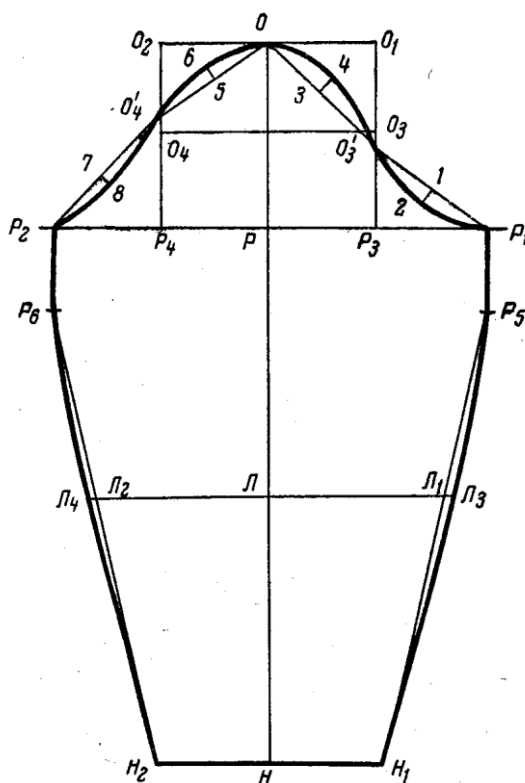
143-rasm. Ayollar jaketining yeng detali chizmasi
