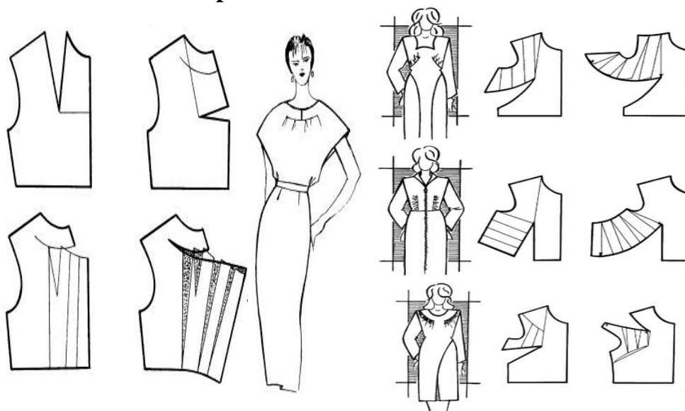
41-rasm. Ayollar kiyimida murakkab burmalar, qirqimlar va drapirovkalar modellashtirish
