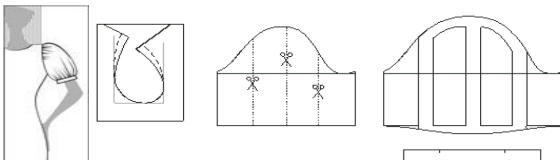
23-rasm. Ayollar kiyimi yengini parallel kengaytirish
