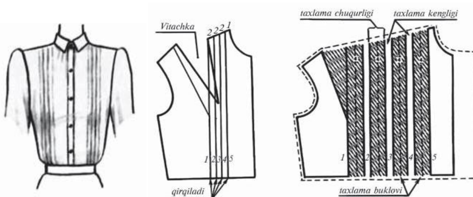
24-rasm. Ayollar bluzasini old detalini parallel kengaytirish va taxlamalar modellashtirish
