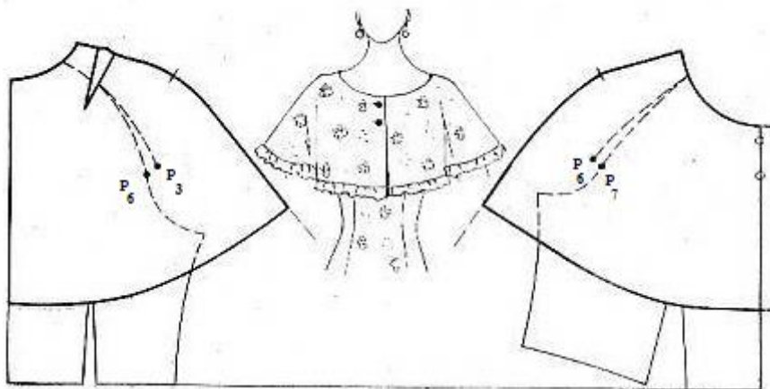
87-rasm. Kichik pelerina
