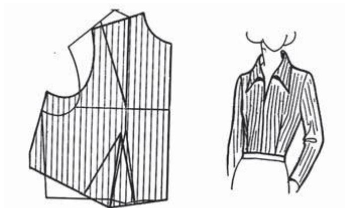
15- rasm. Ko'krak vitochkasini bel chizig'iga ko'chirish
