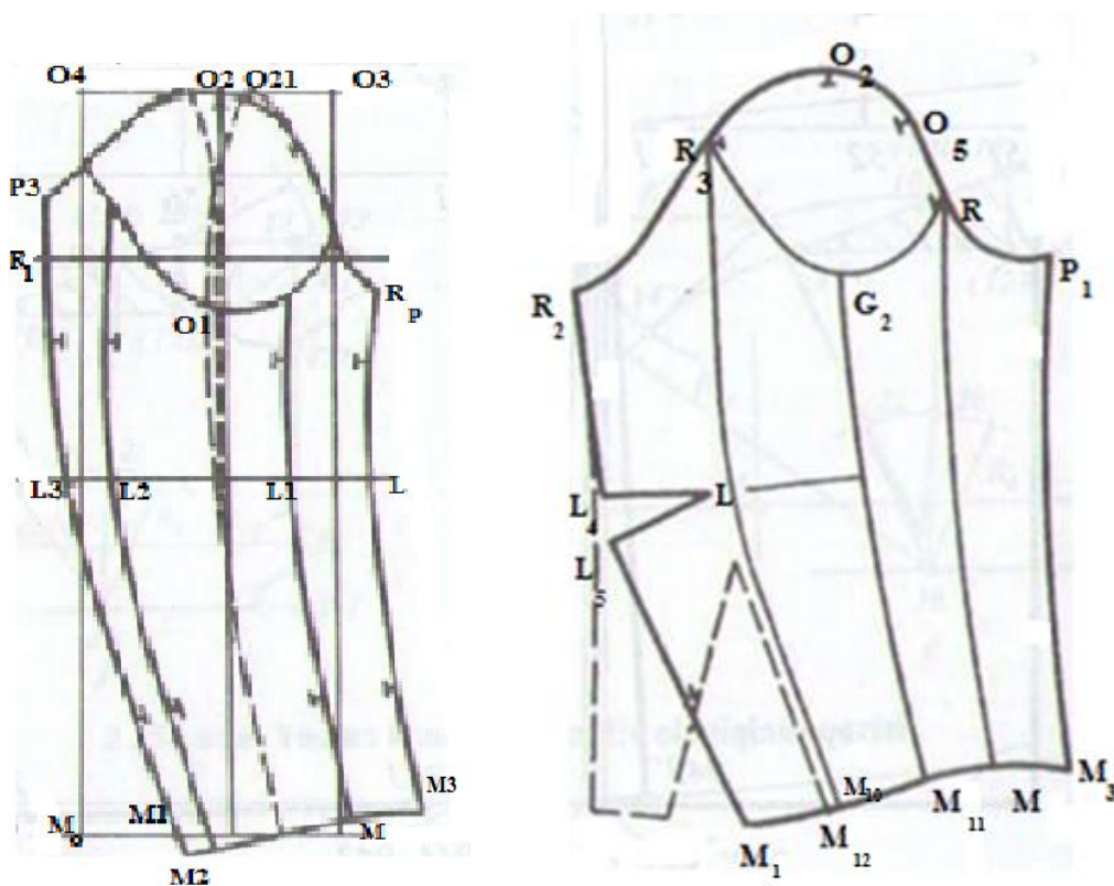
45-rasm. Yeng detallarining sxemalari
