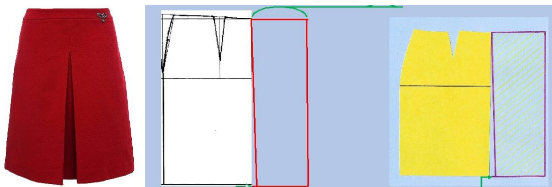
92-rasm. Ayollar yubkasida parallel kengaytirish usuli bilan taxlamalar modellash
