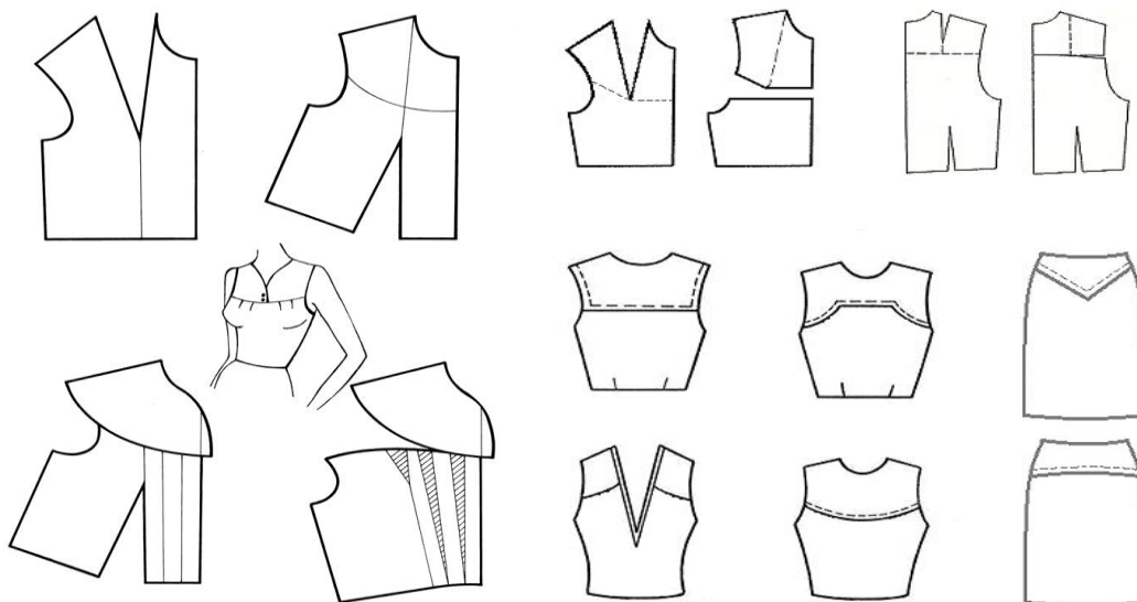
19-rasm. Yelkaga oid va belga oid ayollar kiyimida gorizontaal bo'laklash usulini qo'llab koketkalar modellashtirish
