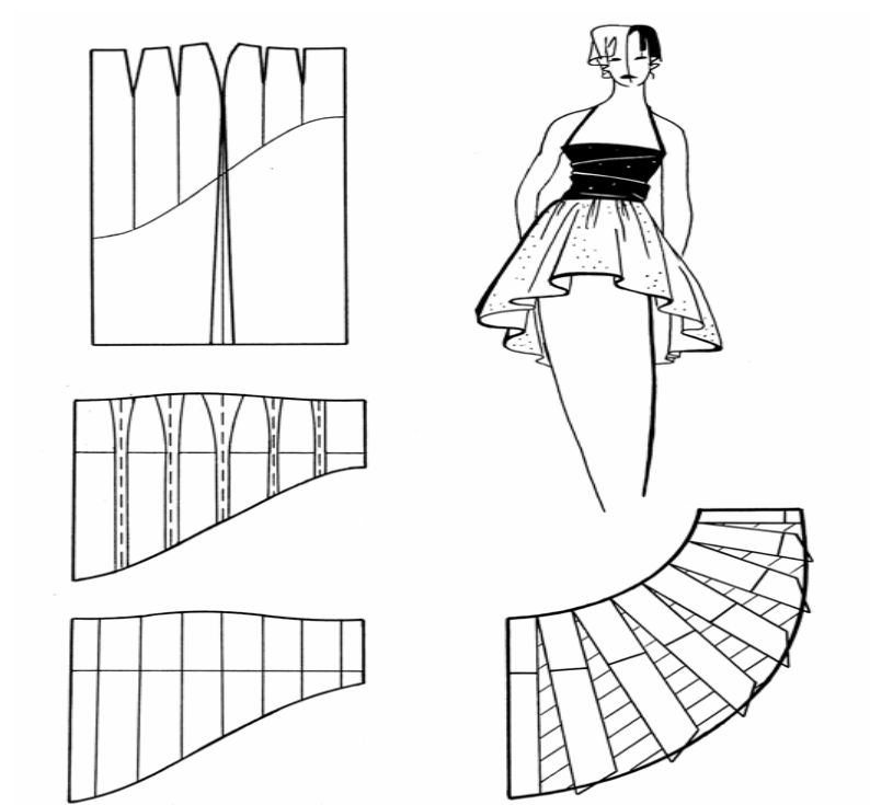
37-rasm. Ayollar yubkasini konussimonsimon kengaytirish
