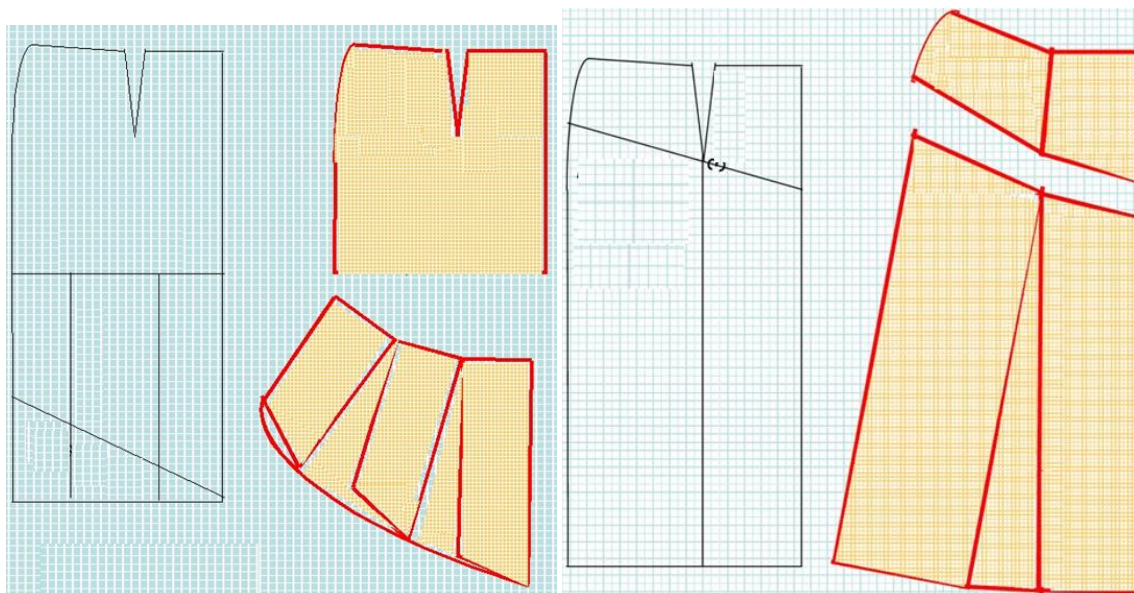
94-rasm. Ayollar yubkasi detallarini gorizontal bo'laklash
