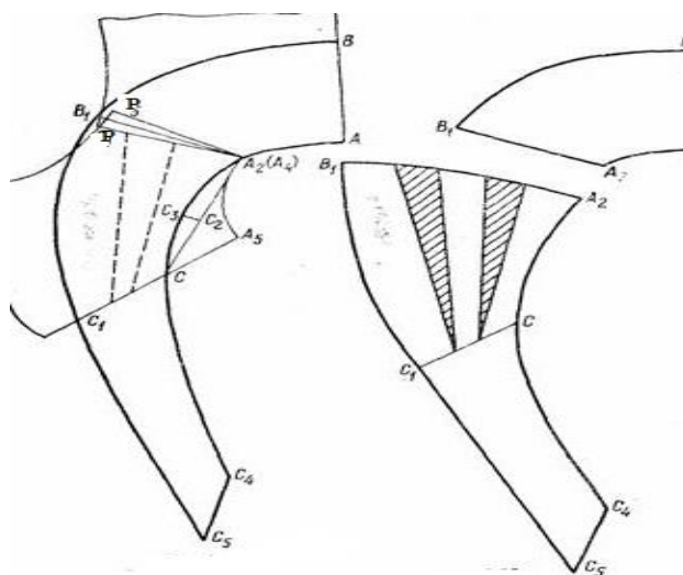
79-rasm. “Kosinka” turidagi bog'lanadigan yoqa chizmasi
