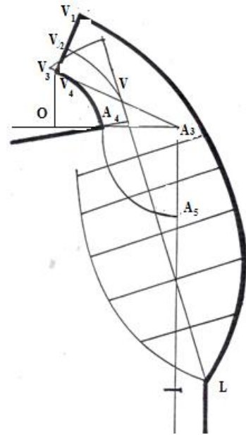
70-rasm. “Shol” tipidagi yoqalar
