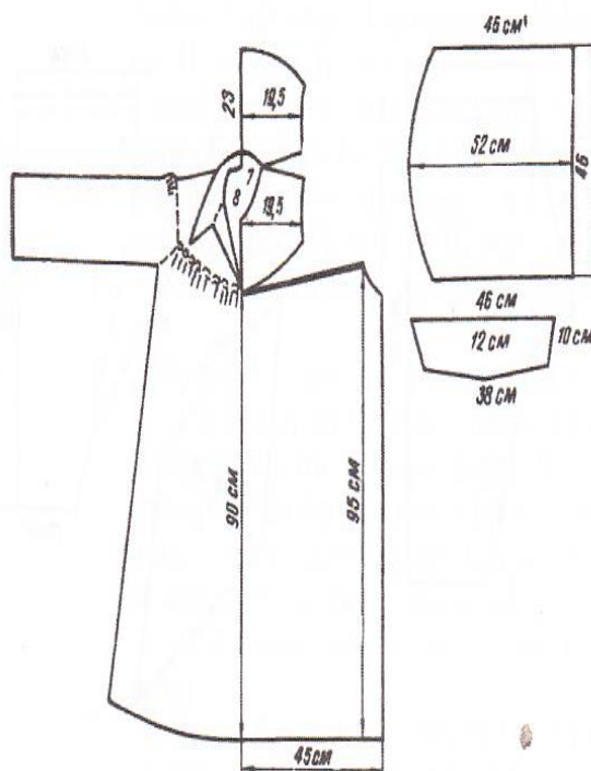
182-rasm. “Ko’krak burma” ayollar ko’ylagining bichimi
