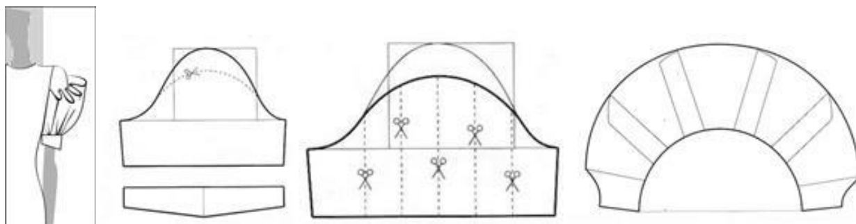
30-rasm. Maketlashtirish usuli bilan hosil qilingan yeng
