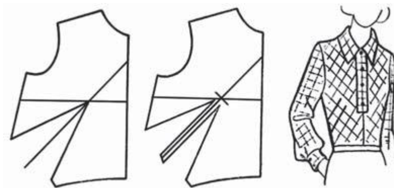
14- rasm. Ko'krak vitochkasini yon qirqim chizig'iga ko'chirish
