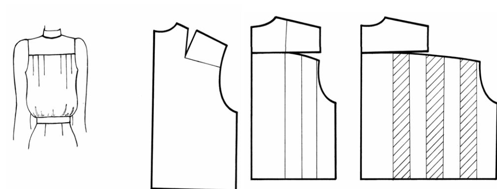
25-rasm. Ayollar bluzasini old detalini parallel kengaytirish va taxlamalar modellashtirish
