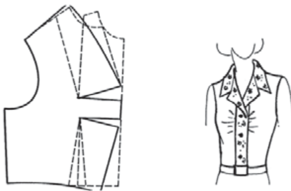
18-rasm. Ko'krak vitochkasini old bo'lak o'rta chizig'iga ko'chirish
