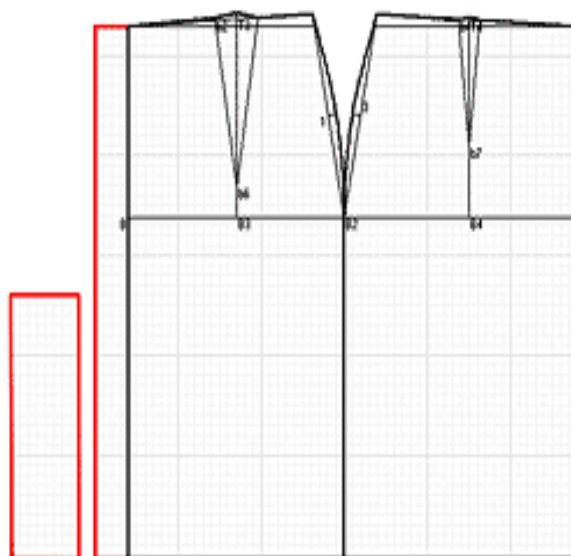
26-rasm. Ayollar ko'ylagining old detalini parallel kengaytirish va taxlamalar modellashtirish
