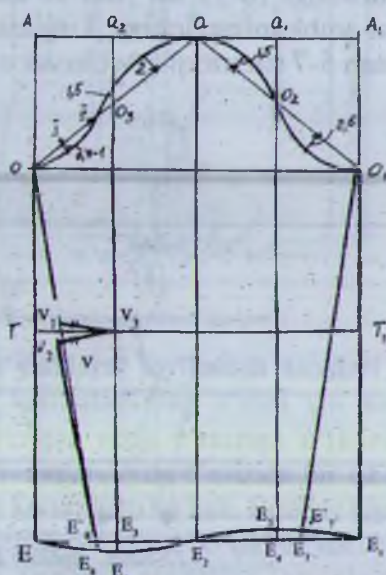
26-rasm. O'tkazma yeng chizmasi
