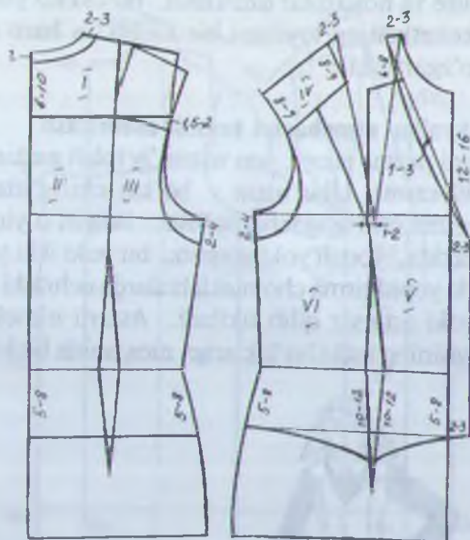
50-rasm. Ayollar nimchasini modellashirish
