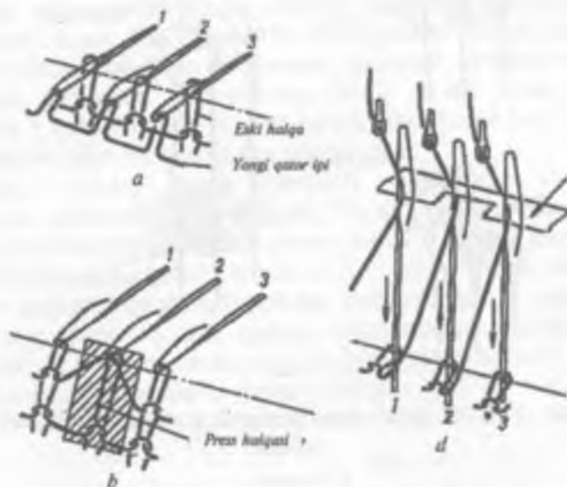
115-rasm. Ilgalki ignali mashinalarda press nabroskasini hosil qilish.
