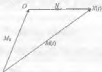
2.19-rasm. Nur.
