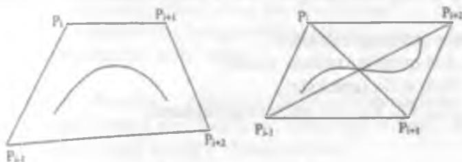
2.13-rasm. B-splayn egri chizig'i.
