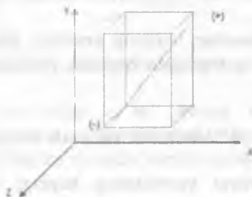
2.20-rasm. Parallelepiped.
