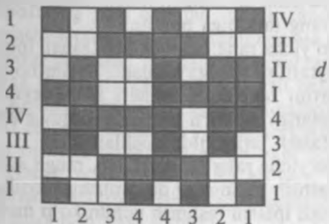
6.6-rasm. Aylantirish usulida krep o'rinishini tuzish.
