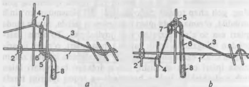
7.14-rasm. O'ramali to'qima ishlab chiqarish uchun xomuza hosil qilish. 1 — zamin tanda ipi, 2 — zamin tanda ipining gulasi, 3 — o'rama tanda ipi, 4 — o'rama shoda gulasi, 5 — qanot shoda gulasi, 6 — yarim qanot gulasi, 7 — murakkab shoda gulasi.
