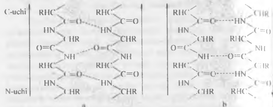
36-rasm. \beta -struktura: parallel (a) va antiparallel (b) zanjirlar
