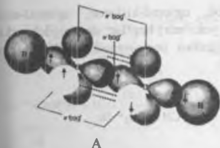
12-rasm. Atsetilen molekulasining tuzilishi
