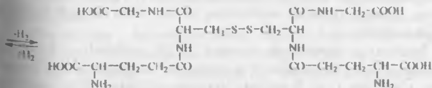
S-S-glutation
