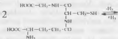
SH-glutation
