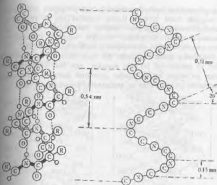
34-rasm. Polipeptid zanjirining \alpha -spirallanishi
