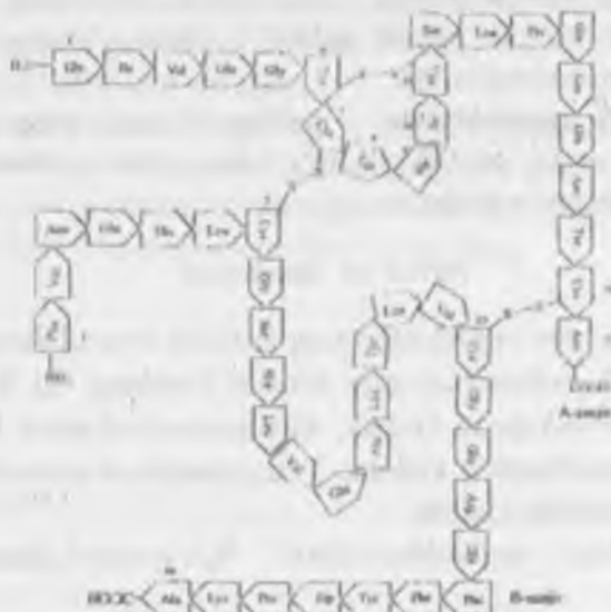
39 -rasm. Insulinning tuzilishi
