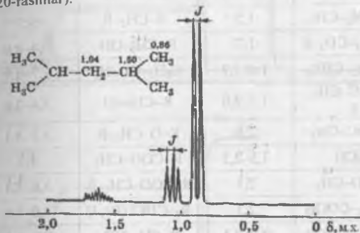
17-rasm. 2,4-dimetilpentanning PMR spektri ( J = 7,6 Gts).
