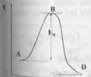
27-rasm. \text{S}_{\text{N}}2 -tipidagi reaksiyaning energetik diagrammasi.
