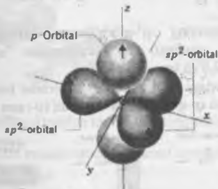
8-rasm. sp^2 -Gibridlangan uglerod atomi
