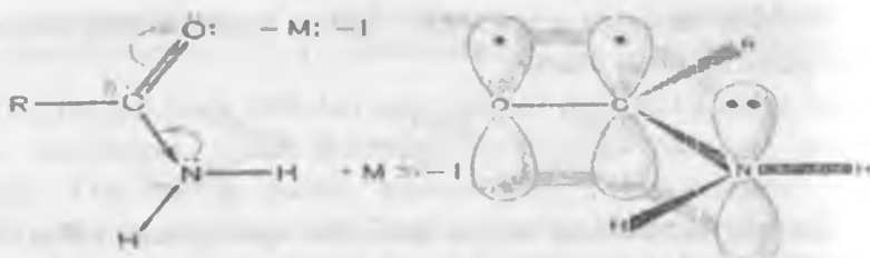
33-rasm. Amid guruhining elektron tuzilishi va p,π-tutashish.
