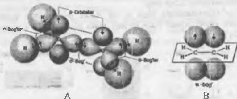
9-rasm. Etilen molekulasining tuzilishi
