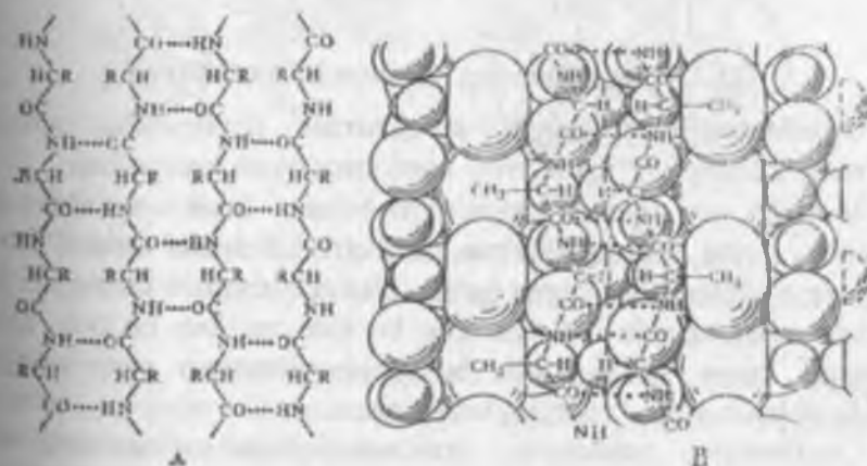
35-rasm. Oqsillarning \beta -strukturasi A – \beta -strukturaning hosil bo‘lishi B – ipak fibroinining tuzilishi
