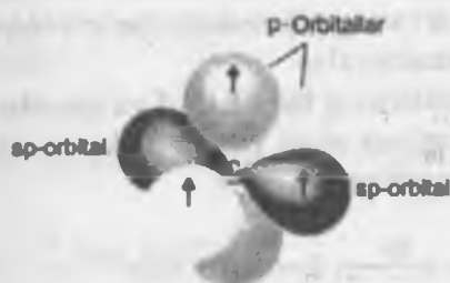
11-rasm. sp -Gibridlangan uglerod atomi
