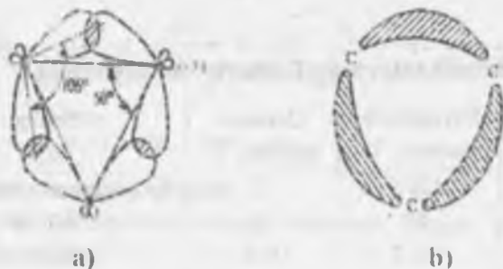
40-rasm. Siklopropanning tuzilishi (a) va "Banan bog'lari" (b)
