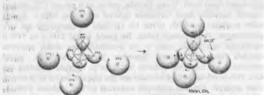
5-rasm. Metan molekulasining hosil bo'lishi
