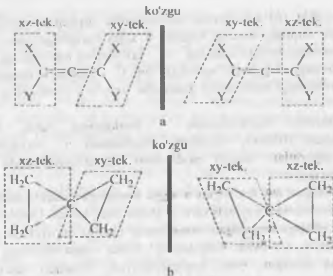
25-rasm. Optik faol allen – (a) va spiro-2,2-pentan – (b).
