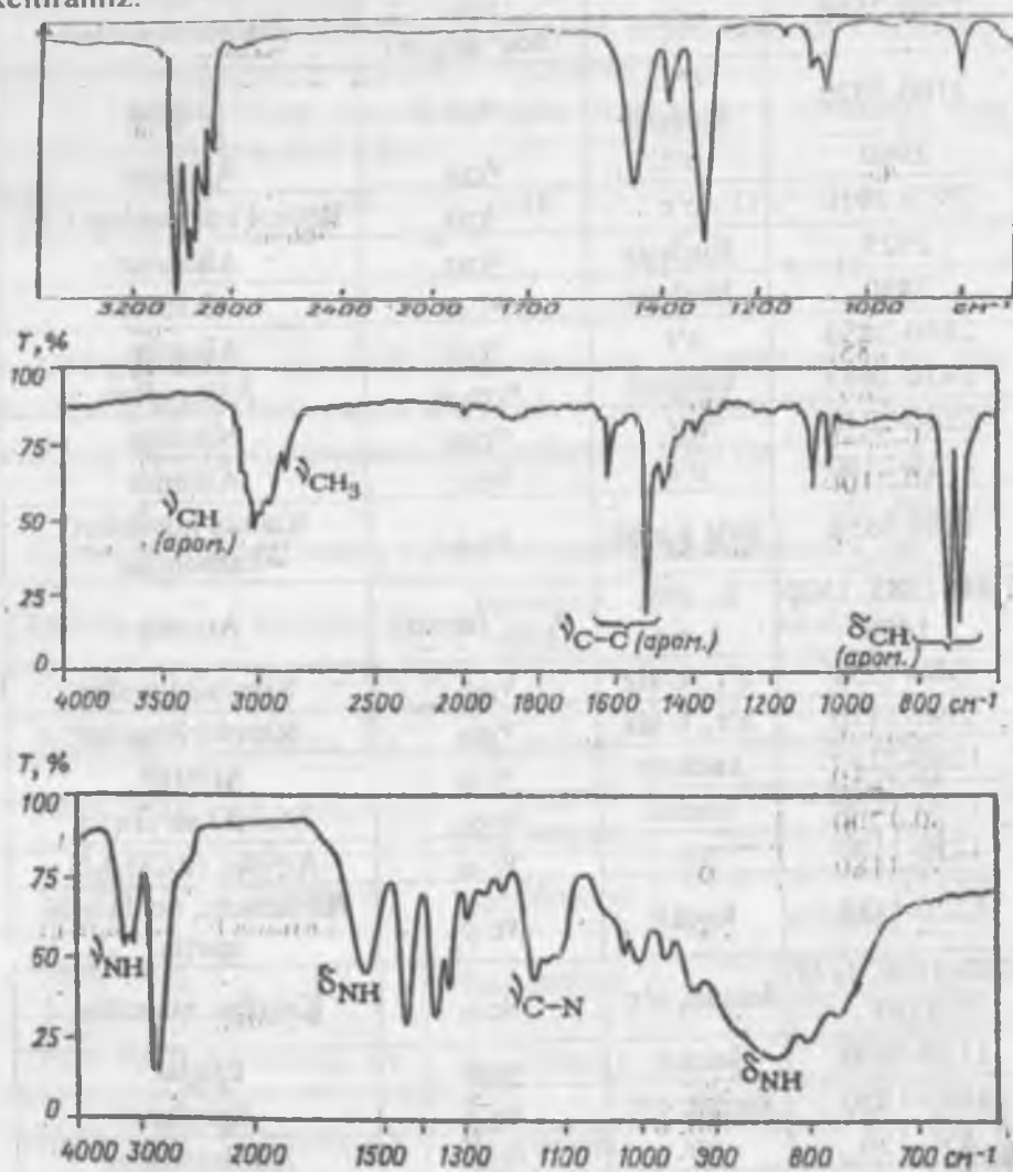
16- rasm. 3-geksinning – (a), toluolning – (b), ikkilamchi butilaminning – (c), IQ spektrlari.
