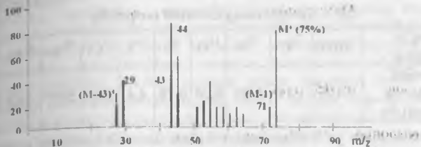
12-rasm. Moy aldegidining mass-spektri.
