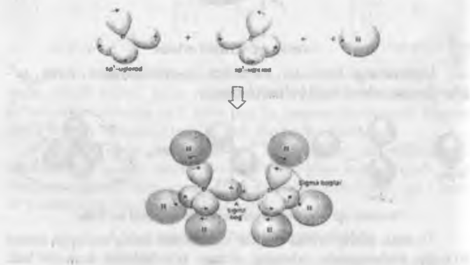
6-rasm. Etan molekulasining hosil bo'lishi
