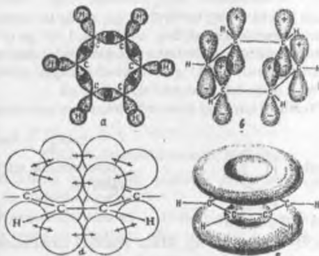
42-rasm. Benzol molekulasining tuzilishi.
