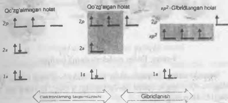
7-rasm. Uglerod atomining sp^2 -gibridlanishi
