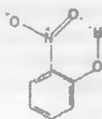
o-nitrofenol
