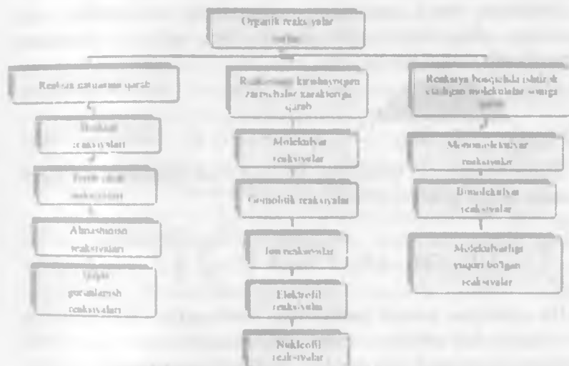
3.1-Rasm. Organik reaksiyalarining sinflanishini
