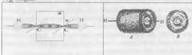
1.9-Rasm. Atsetilen molekulasidagi sp^2 - gibridlanishi
