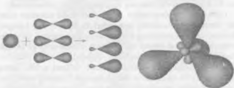
1.3-Rasm. Uglerodning bitta s va uchta p - orbitalaridan to'rtta gibriz orbitalning hosil bo'lishi
