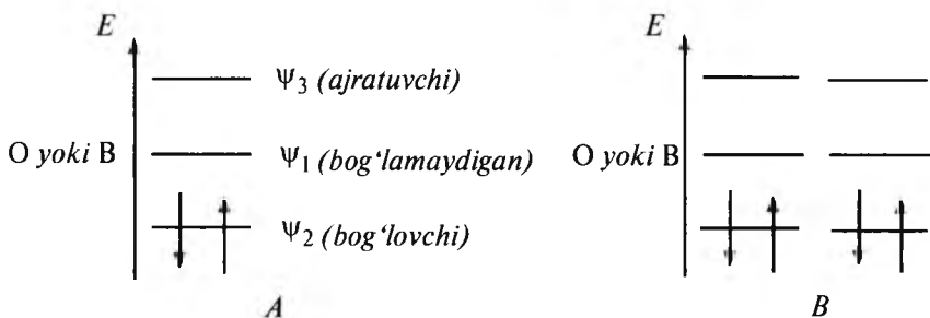
2.32-rasm. H \cdots B \cdots H (A) va B \begin{array}{c} H \\ \diagup \quad \diagdown \\ B \quad B \\ \diagdown \quad \diagup \\ H \end{array} (B) fragmentlarning
