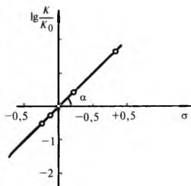
4.22-rasm. \lg K/K_0 ning u ga bog'liqligining almashingan benzoy kislotalar dissotsiatsiyasi misolida ifodalanishi t=25^\circ\text{C} ; erituvchi-suv; s=1,0 ; \lg K_0=-4.203 .
