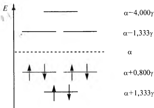
2.35-rasm. Benzol molekulasida uchun s \neq 0 deb qarab hisoblab topilgan MO lar va ularning energetik pog'onalari.
