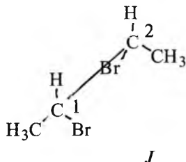
Treo(trans)-2,3-dibrombutan
