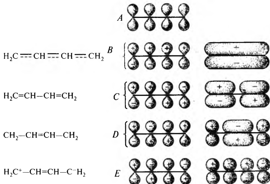
3.2-rasm. Butadiyen molekulasining orbitallari.
