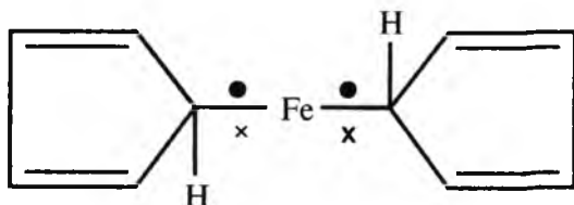
3.24-rasm. Ferrosen molekulasining tuzilishi (A, B).
