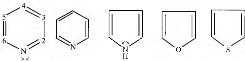
Piridin
