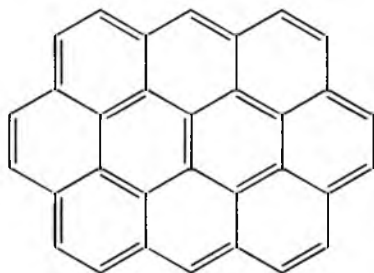
Ovalen
