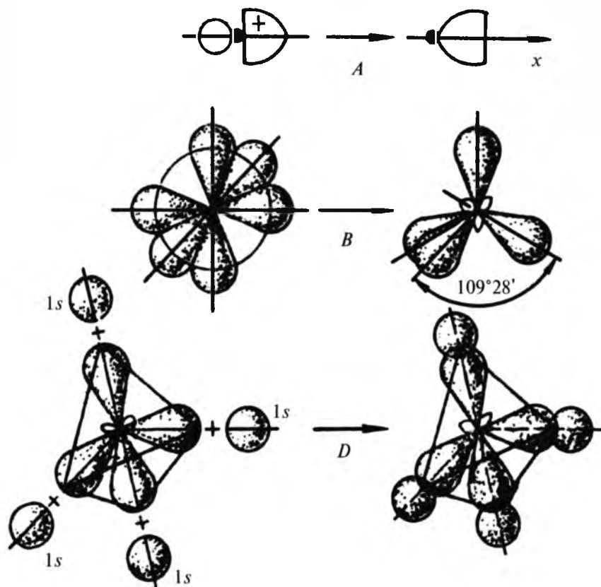
2.40-rasm. A — gibril orbital; B — s - va p - orbitallardan uglerodning gibril orbitallarining yuzaga kelishi; D — metan molekulasi hosil bo'lishi.
