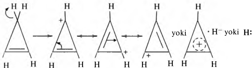
Tsiklopropeniliiy-kation
