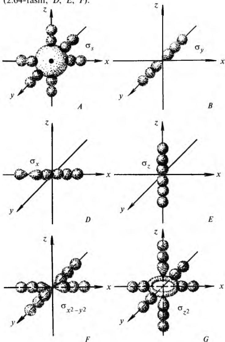
2.64-rasm. [\text{Me}(\text{H}_2\text{O})_6]^{n+} tarkibli kompleksda bog'lovchi MO larning hosil bo'lishi.
