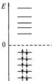
3.12-rasm. Naftalin molekulasini MO larining energetik pog'onolari
