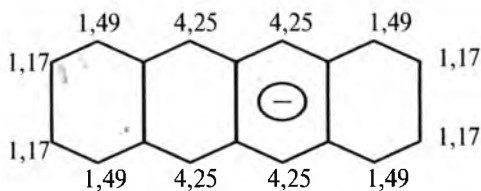
Tetratsen anion-radikali
