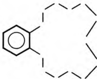
Monobenzo-15-kraun-5
