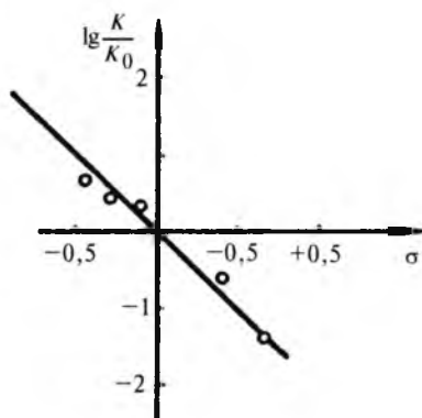
4.23-rasm. Benzil xloridning suv ta'sirida gidrozlanish jarayoni uchun Gammet tenglamasi chizma ifodasi ( t=30^\circ\text{C} ; erituvchi-47% li etil spirt; s=-2,20 ; \lg K_0=5,61 ).
