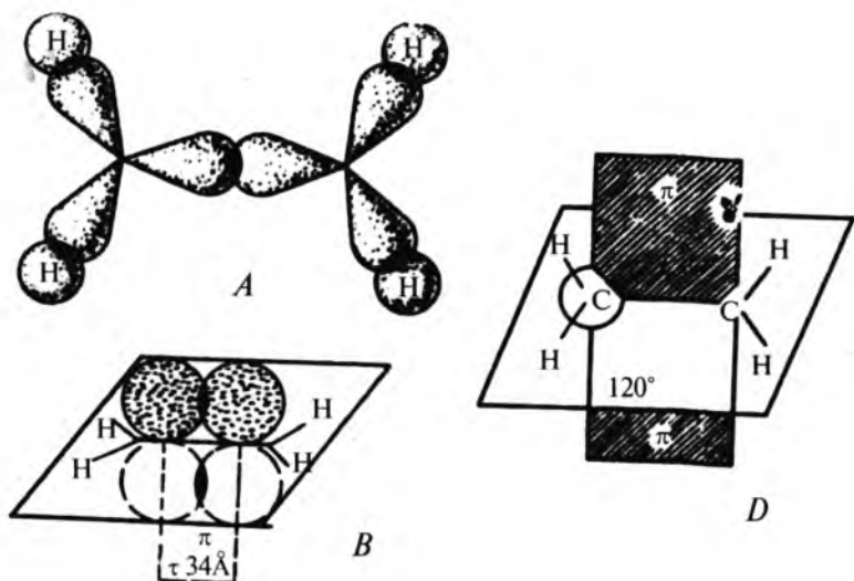
2.48-rasm. Etilen molekulasining hosil bo'lishi.
