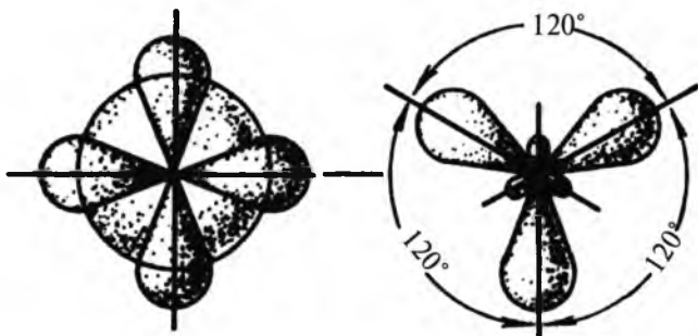
2.47-rasm. sp^2 -gibrirlanish orbitalarining hosil bo'lishi.
