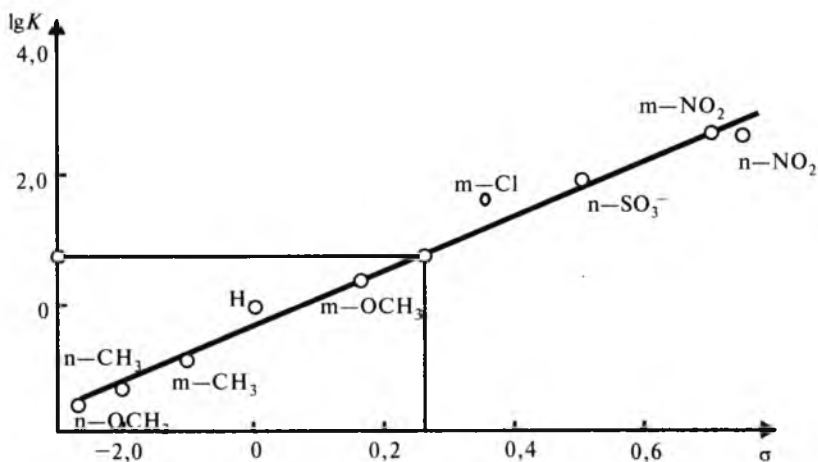
4.25-rasm. Meta- va para- \text{X-C}_6\text{H}_4\text{-N}_2 bilan 2,6-naftalin disulfokislota o'rtasida boradigan reaksiyalar tezlik konstantalari logarifmining u bilan bog'liqligi ( \rho=+4,26 ).
