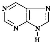
purin
