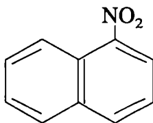
\alpha - nitronaftalin
