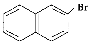
\beta - bromnaftalin
