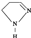
2 –pirazolin
