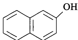
\beta - naftol
