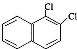
o-dixlor-naftalin
