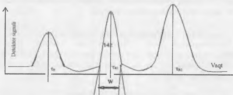
14.1-rasm. Xromatogramma
