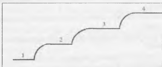
17.1-rasm. Derivatogramma (termoliz egri chizig'i)
