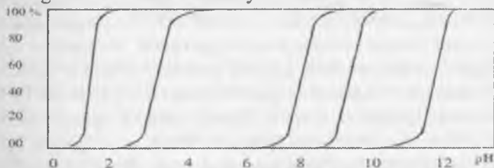
13.1-rasm. Ekstraksiya darajasining Hg^{2+} , Bi^{3+} , Pb^{2+} , Zn^{2+} , Cd^{2+} ditizonatlarining (mos ravishda) xloroformda ajralishining pH ga bog'liqligi
