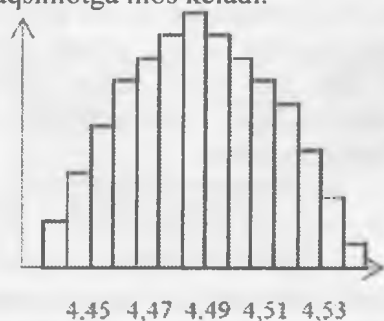
3.2-rasm. Variatsiyalar taqsimoti
