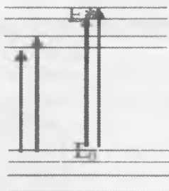
24.1-rasm. Molekulaning energetik sathlari
