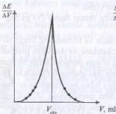
10- rasm. Potensiometrik titrlashning differensial egri chizig'i.
