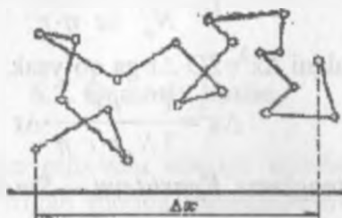
Zarrachaning Broun harakati sxemasi.
