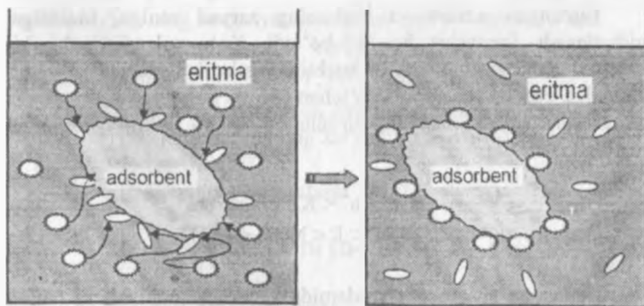
Rasm. Almashinish adsorbsiyasi sxemasi
