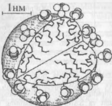
SAM to'g'ri mitsellasining sferik shakli
