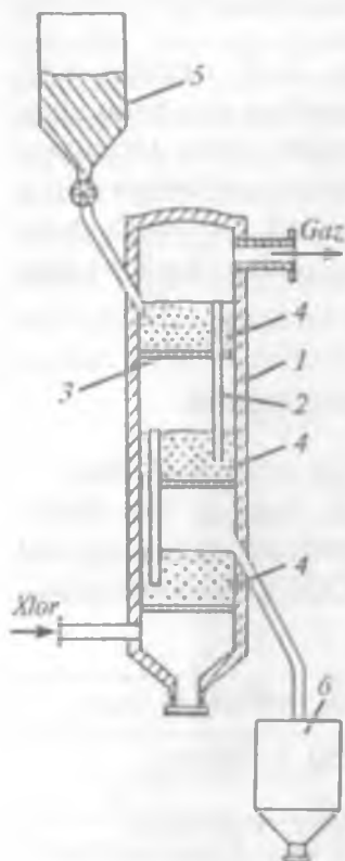
1-rasm. Qaynovchi qavatlarida xlorldash.
