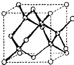
40-rasm. Olmos kristall panjarasining tuzilishi.
