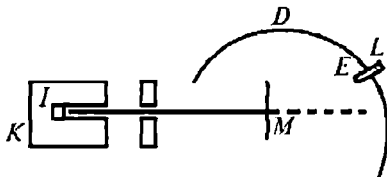
5- rasm. \alpha - zarrachalarning yupqa metallar pardadan o'tishi.
