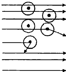
6-rasm. \alpha - zarrachalarning metalldan o'tishida og'ishi.
