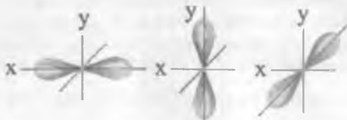
Uchta p – orbital
