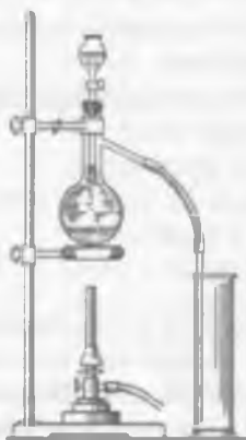
15-rasm. Xlor olish asbobi.
