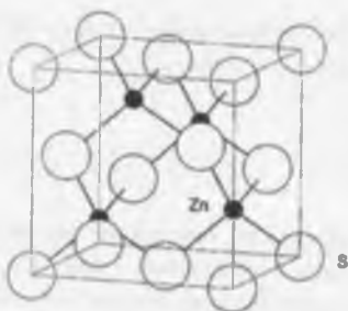
Fig. 2.9 Zinc blende structure.
