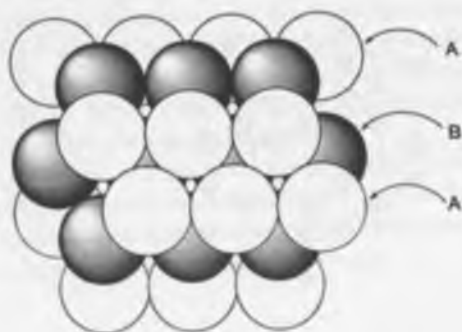
Fig. 2.2 Hexagonally close-packed (hcp) of balls.
