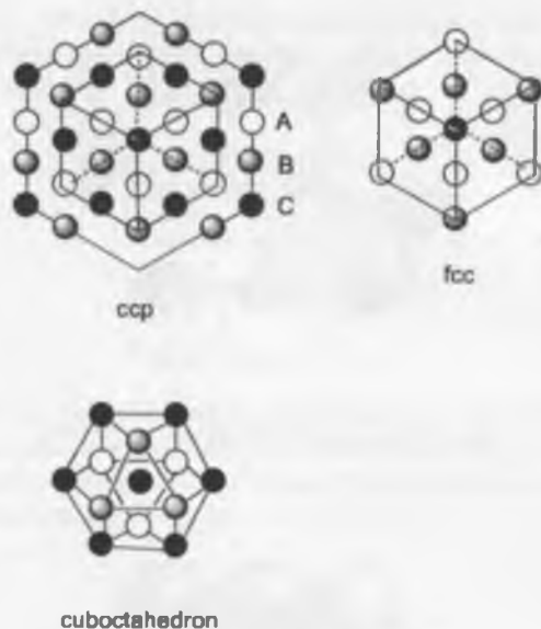
Fig. 2.4 Different expressions of cubic close-packed
