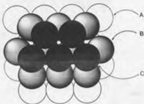
Fig. 2.3 Cubic close-packed (ccp) of balls.
