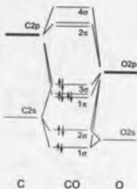
Fig. 2.22 Molecular orbitals of CO.
