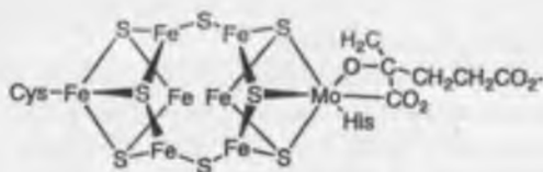
Figure 8.2 Structure of Fe-Mo cofactor in nitrogenase.
