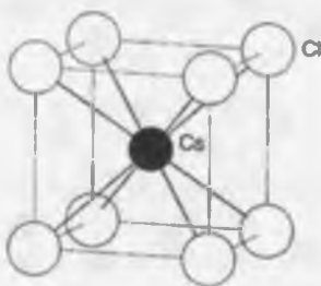
Fig. 2.8 Cesium chloride structure.
