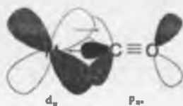
Fig 6.15 Back donation in metal carbonyls.
