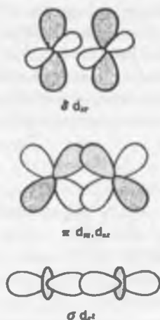
Fig. 6.22 Overlap of d orbitals in \text{Re}=\text{Re} quadrupole bond.
