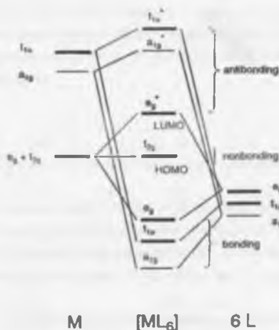
Fig. 6.10 Bonding and anti-bonding M(metal)-L(ligand) molecular orbitals.
