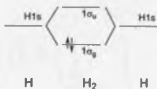
Fig. 2.18 The molecular orbitals of H 3 . The arrows indicate the electron spins.
