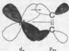
Fig. 6.17 Back-donation in olefin complexes.
