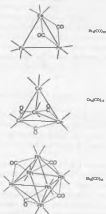
Fig. 6.23 Examples of metal cluster carbonyls (terminal carbonyl ligands are omitted for clarity).
