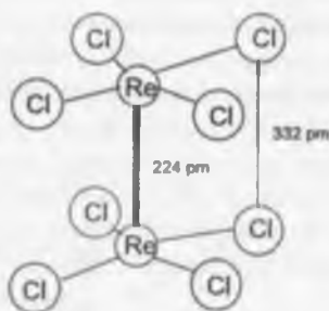
Fig. 6.21 Structure of \text{Re}_2\text{Cl}_8^{2-} .
