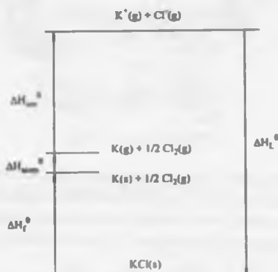
Fig. 2.1 Born-Haber cycle of KCl.
