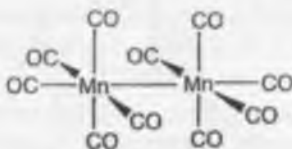
Fig. 6.20 Structure of \text{Mn}_2(\text{CO})_{10} .
