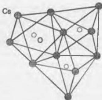
Fig. 4.12 Structure of \text{Cs}_{11}\text{O}_3 .
