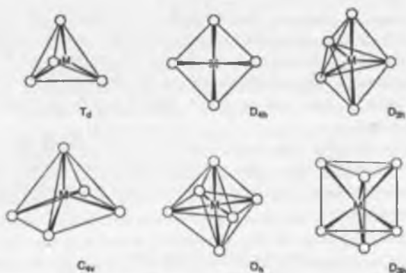
Fig. 6.1 Structure of 4 – 6 coordination.
