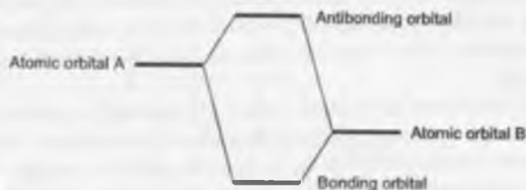
Fig. 2.15 Construction of molecular orbitals.
