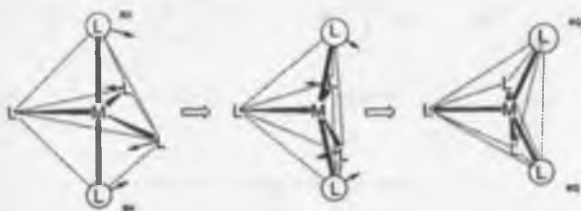
Fig. 6.2 Berry's pseudorotation.
