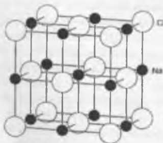
Fig. 2.7 Rock-salt structure.
