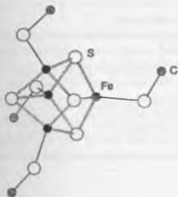
Fig. 6.25 Structure of [\text{Fe}_4\text{S}_4(\text{SR})_4]^{2-} .
