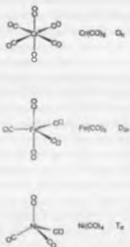
Fig. 6.14 Structures of metal carbonyl compounds.
