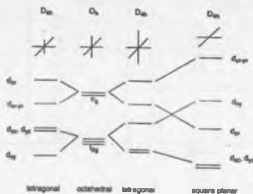
Fig. 6.7 Change of the orbital energy from octahedral to square planar complexes.
