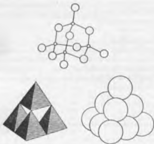
Fig. 2.12 Three expressions for the structure of P_4O_{10} .
