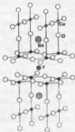
Figure 8.4 Structure of YBa 2 Cu 3 O 7-x .
