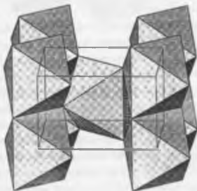
Fig. 4.13 Structure of rutile.
