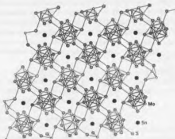
Fig. 4.20 Structure of SnMo_6S_8 .
