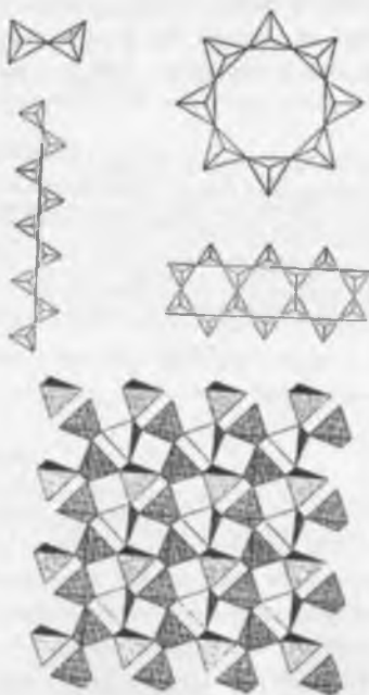
Fig. 4.9 Bridging modes of the \text{SiO}_4 tetrahedra.
