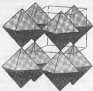
Fig. 4.14 Structure of \text{ReO}_3 .
