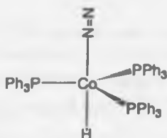
Fig. 6.19 Structure of [\text{CoH}(\text{N}_2)(\text{PPh}_3)_3] .
