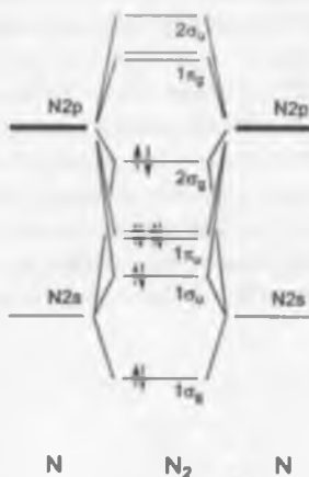
Fig. 2.19 Molecular orbitals of N 2 .
