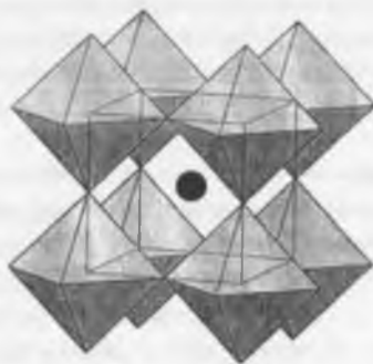
Fig. 4.16 Perovskite structure.
