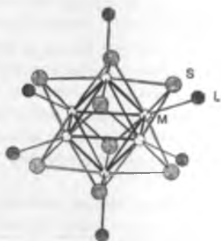
Fig. 6.24 Structure of [\text{Mo}_6\text{S}_8\text{L}_6] .
