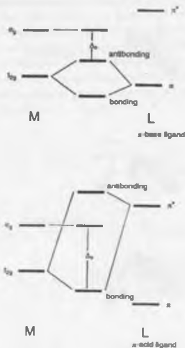
Fig. 6.12 The energy change upon formation of M-L \pi bonds.
