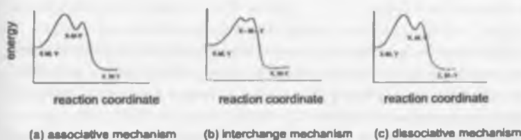
Fig. 6.26 The stability of the intermediate of ligand substitution.
