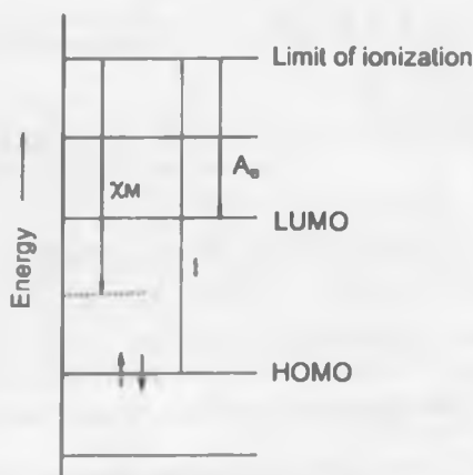
Fig. 2.14 Mulliken electronegativity.
