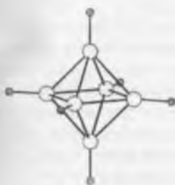
(a) closo - [B_6H_6]^{2-}
