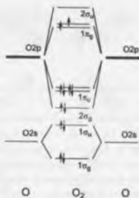
Fig. 2.20 Molecular orbitals of O_2 .
