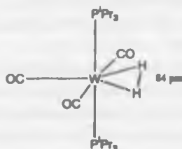
Fig. 6.18 Structure of [\text{W}(\text{CO})_3(\text{H}_2)(\text{P}^i\text{Pr}_3)_2] .
