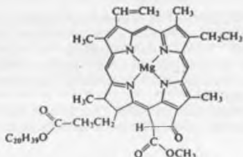
Figure 8.3 Chlorophyll a.
