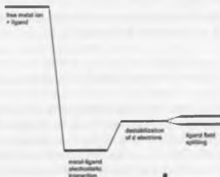
Fig. 6.4 Change of electronic energy upon complex formation.
