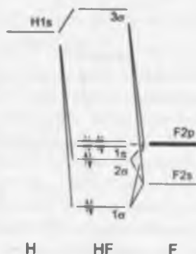
Fig. 2.21 Molecular orbitals of HF.
