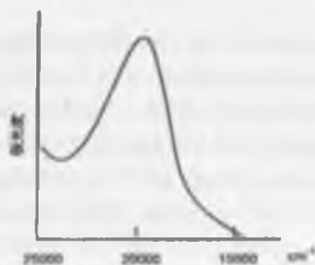
Fig. 6.13 A visible absorption spectrum of [\text{Ti}(\text{OH}_2)_6]^{3+} .
