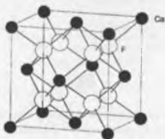
Fig. 2.10 Fluorite structure.
