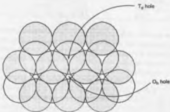
Fig. 2.6 Octahedral and tetrahedral holes.
