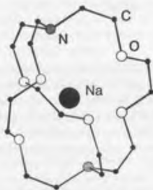
Fig. 5.1 Structure of Na(crypt).
