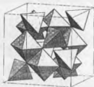
Fig. 4.15 Spinel structure.
