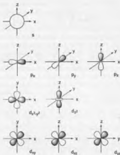
Fig. 1.1 Shapes of s, p, and d orbitals.
