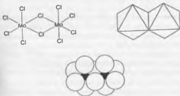
Fig. 2.13 Three expressions for the structure of Mo_2Cl_{10} .
