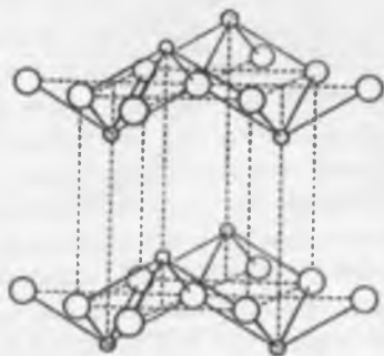
Fig. 4.11 Structure of \text{PbO} .
