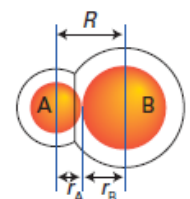
18 Covalent radius
