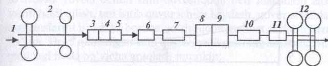
22- rasm. Issiq magistral quvurning texnologik chizmasi:
