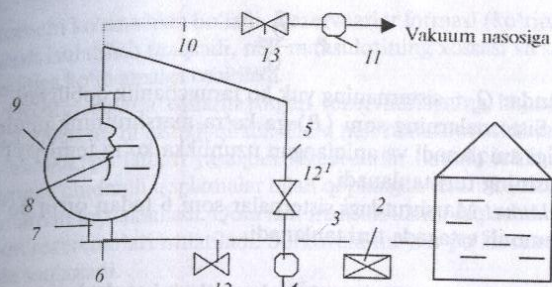
37- rasm. Nasos yordamida to'kish va quyish chizmasi:
