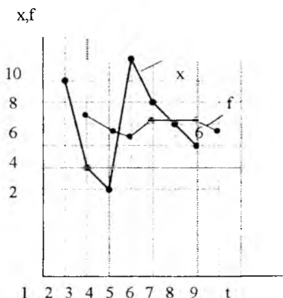
2.9-rasm. Vaqtinchalik bashorat ( x ) va ( f ) eksposial pasayish usulida
