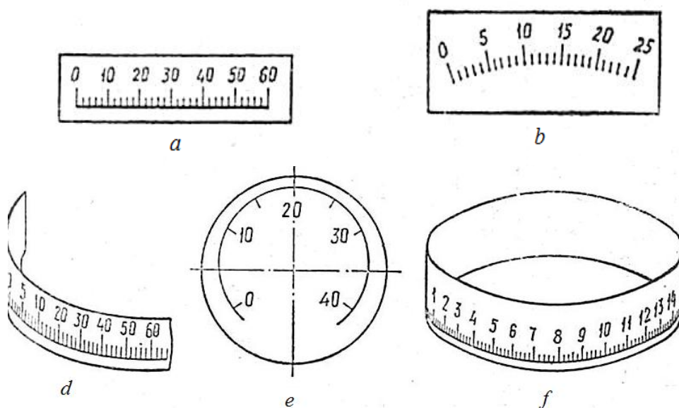
1.4- rasm. Shkalalar: a - to'g'ri chiziqli; b - yoysimon (yoy burchagi 180° gacha); d - yassi; e - yoysimon (yoy burchagi 180° dan yuqori), f -silindrsimon
