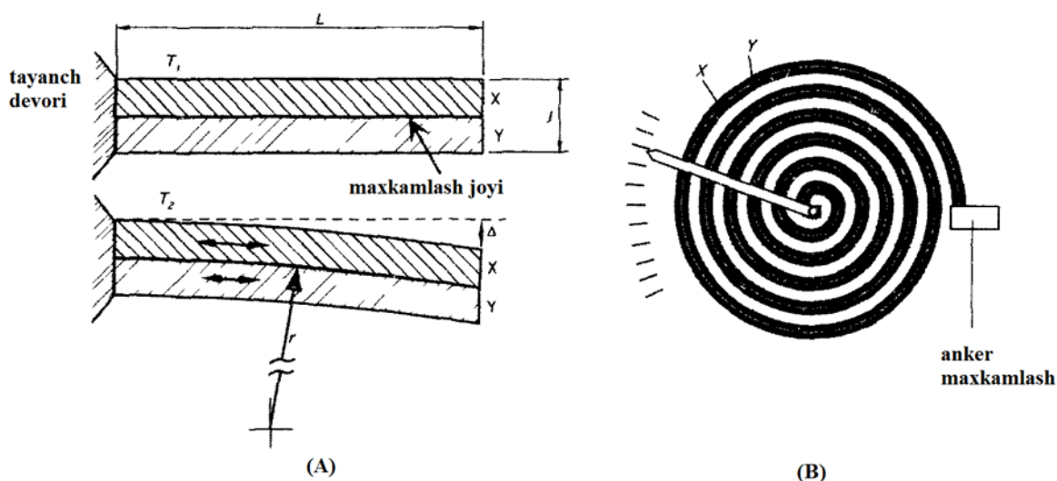
4.23- rasm. A – ikki qatlamli strukturaning egilishi, B – harorat datchigi sifatida foydalaniladigan biometall spiral
