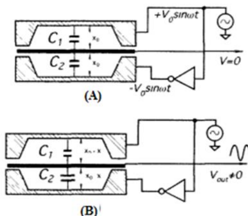
5.11- rasm. Yassi plastinkali sig'imli datchikning harakat tamoyili: A – muvozanatlangan holat; B – muvozanatlanmagan holat
