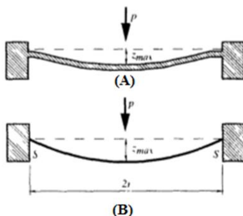
5.23- rasm. (A) -bosim ostida yupqa plastinkaning; (B) -membrananing deformatsiyalanishi
