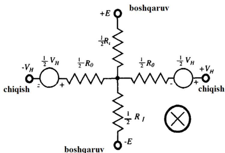
4.18- rasm. Xoll datchigining ekvivalent sxemasi
