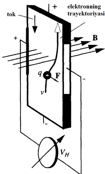
4.16- rasm. Xoll datchigi
