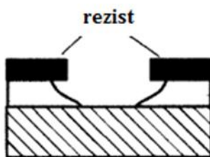
4.43- rasm. Niqob qatlami ostida izotrop eritish
