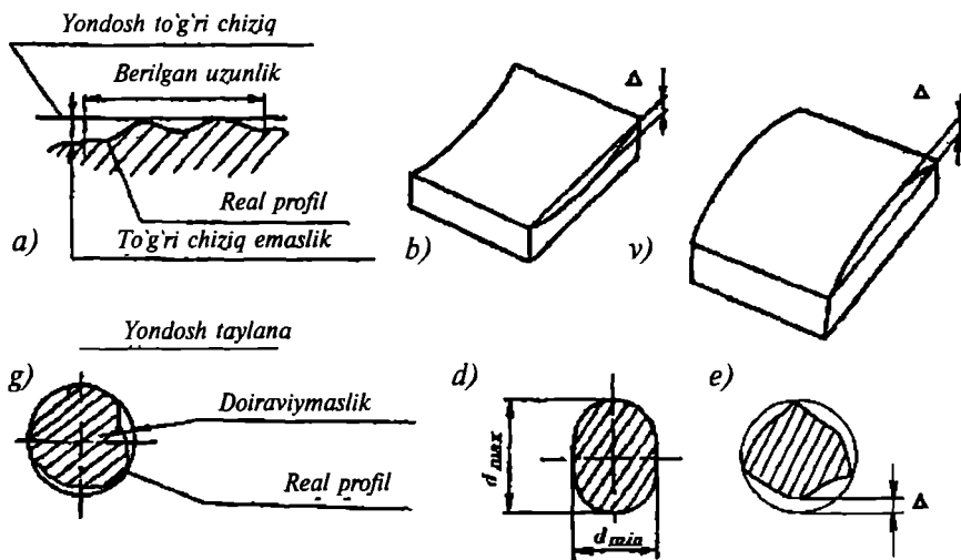
4-rasm. Shakl og'ishi.
