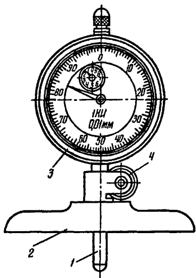
40-rasm. Indikatorli glubinomer:
