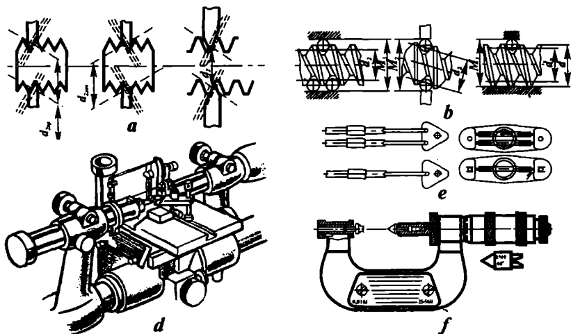
6.15-rasm. Tashqi rezbaning o'rtta diametrini o'lchash sxemalari:
