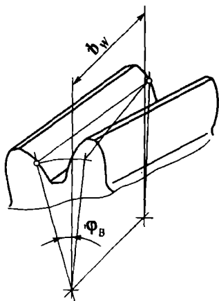
7.9-rasm. Tojning ishchi-eni b_w dagi o'q bo'ylab o'zaro qoplanish burchagi \phi_p .
