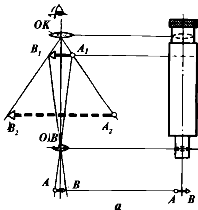
1.29-rasm. БМИ asbob mikroskopi:
