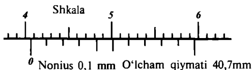
1.5-rasm. Shkala va nonius bo‘yicha o‘lchash.
