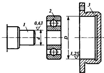
3.11-rasm. Podshipnik uzelinesi detallari.
