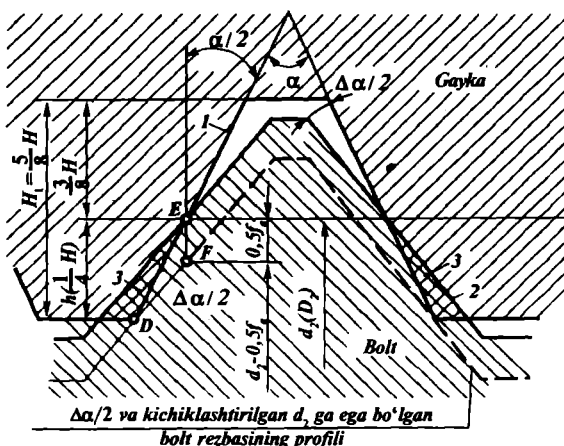
6.5-rasm. Profil burchagi yarmining o'g'ishi \Delta\alpha/2 va uning diametral kompensatsiyasi f_\alpha .
