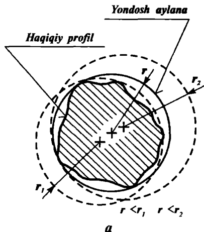
5.3-rasm. Yuzalarning yumaloqligidan og'ishi:
