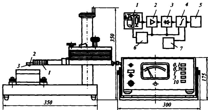
5.38-rasm. Mexatronli profilometr:
