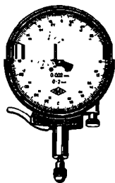
1.16-rasm. Ko'p aylanishli pishang-tishli kallak МИГ.
