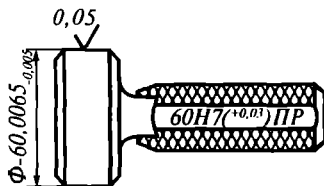
3.23-rasm. Silliq o'tuvchi kalibr.
