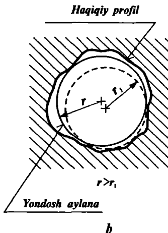
5.3-rasm. Yuzalarning yumaloqligidan og'ishi:
