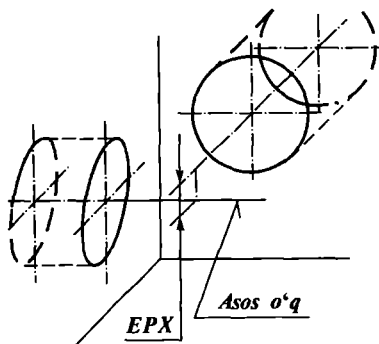
5.21-rasm. O'qlarning kesishmasidan og'ish.
