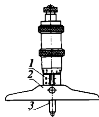
1.10-rasm. Mikrometrik chuqurlik o'lchagichi.
