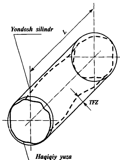
5.2-rasm. Silindrlilikdan og'ish.
