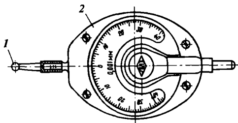
1.21-rasm. Pishang prujinali o'lchash kallagi (minikator).
