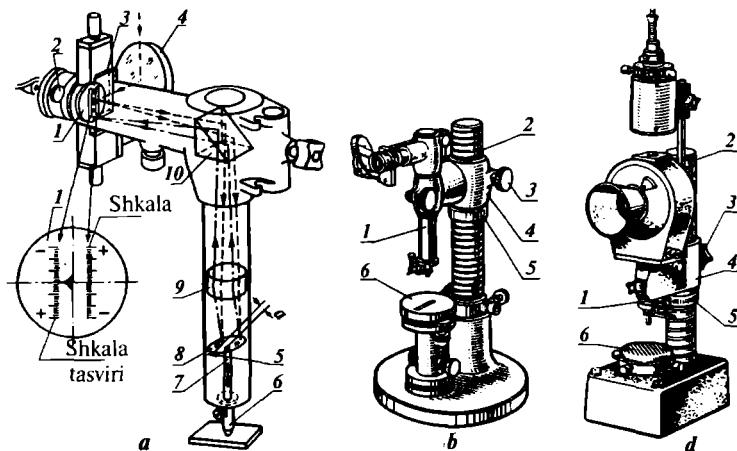
1.25-rasm. Optimetr:
