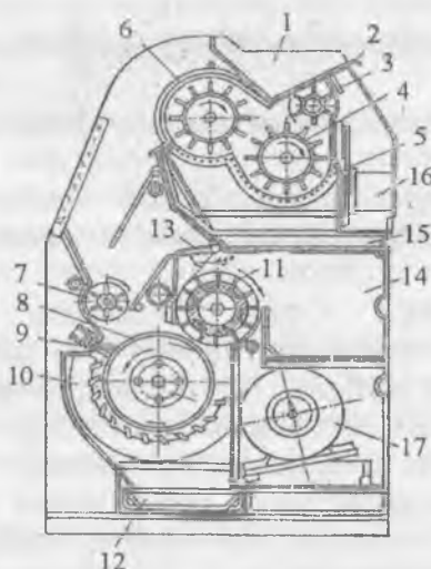
11-rasm. LKM rusumli asbob chizmasi:
