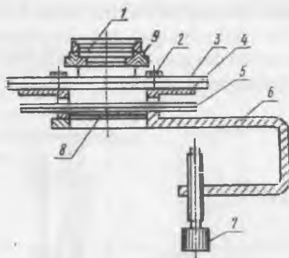
20-rasm. P-2 qutblashtirish moslamasi
