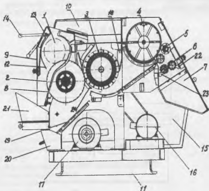
13-rasm. DL-10 laboratoriya jini:
