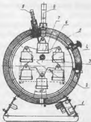
7 -rasm Uz-7M quritish shkafining chizmasi:
