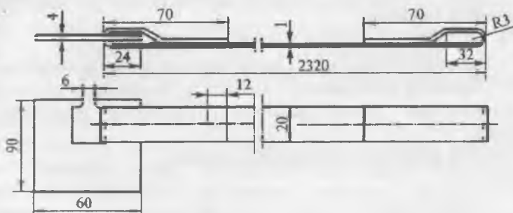
40-rasm. Ilgakli tasma chizmasi
