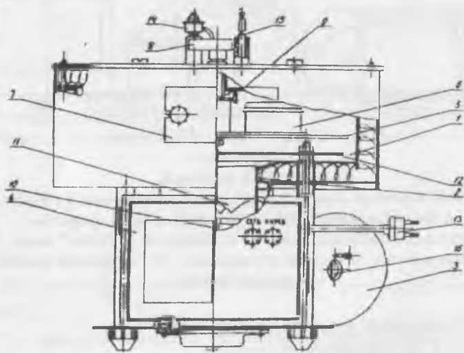
9-rasm. SHSX-1 quritish shkafining chizmasi:
