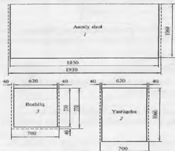
38-rasm. Shollarni bichish sxemasi
