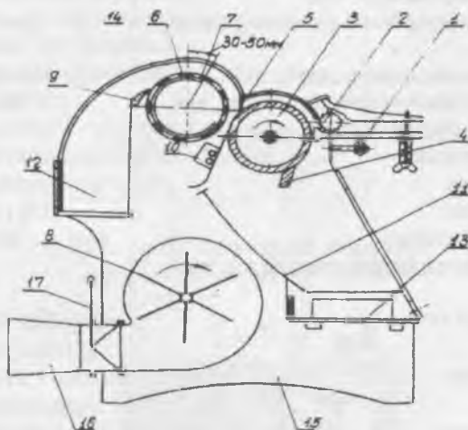
15-rasm AX-2 paxta analizatorining chizmasi:
