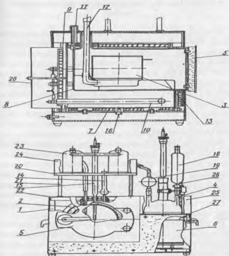
36-rasm. OSX - 1 chigit tuksizlantirgichning chizmasi:
