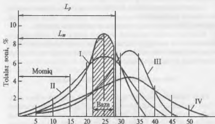
29-rasm. Paxta tolarining uzunligi jihatidan taqsimlanish diagrammasi
