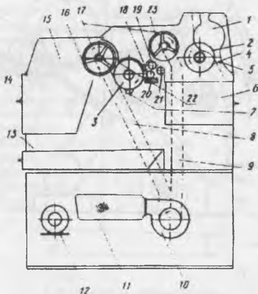
12 - rasm. PPV jin - tola tozalagichning chizmasi:
