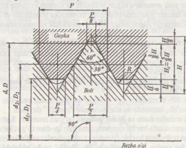
34-rasm. Metrik rezbaning profili.
