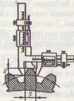
50-rasm. Shtagentish o'lchagich.
