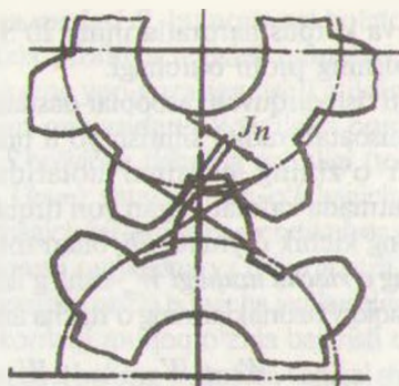
48-rasm. Yon tirqish.
