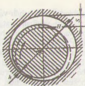
13-rasm. Val — sirpanish podshipnigi birikmasida val holati.
