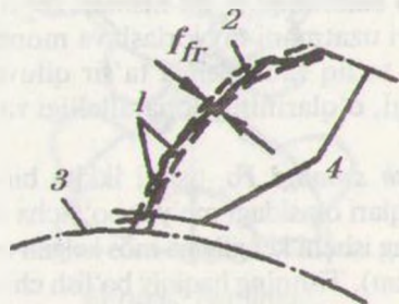
45-rasm. Tish profilining xatoligi:
